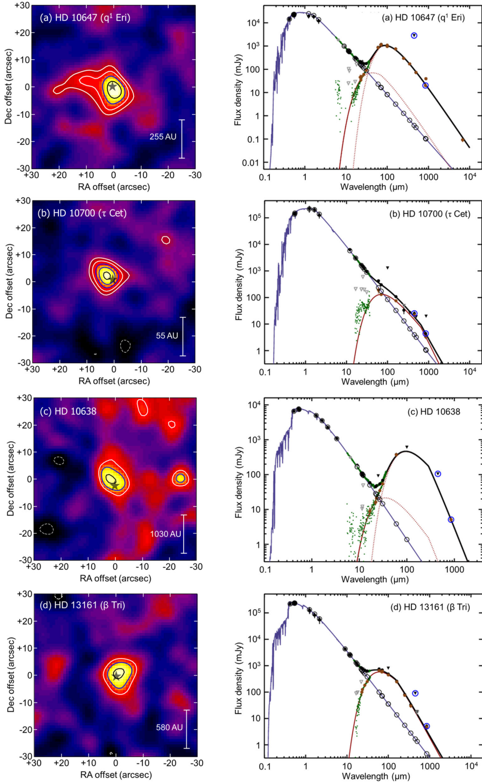
Figure A2. As for Fig. A1 for the targets (a) HD 10647 ( q^1 Eri), (b) HD 10700 ( \tau Cet), (c) HD 10638 and (d) HD 13161 ( \beta Tri).
