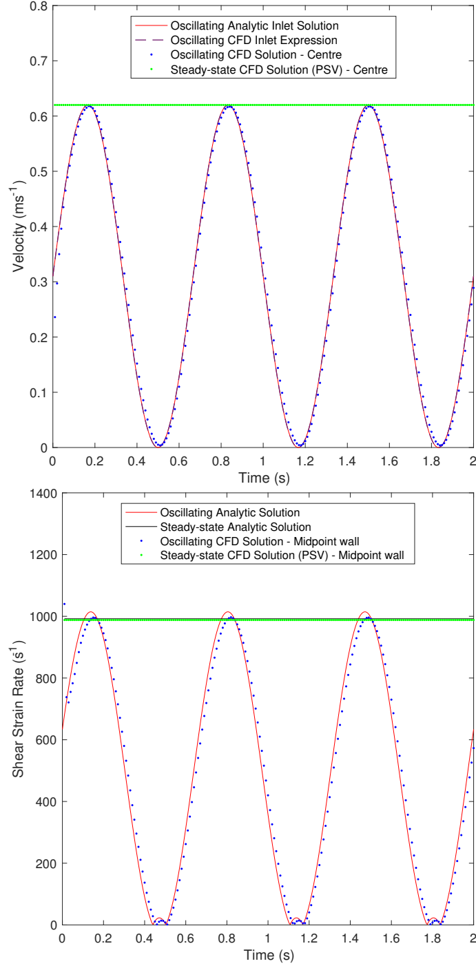
Figure 6: Pristine vessel verification - analytic and CFD sinusoidal pulse, and steady-state (PSV) CFD data (Velocity ( top ) & SSR ( bottom ) where SSR_{max} is plotted for steady-state, and SSR_t for transient cases).
