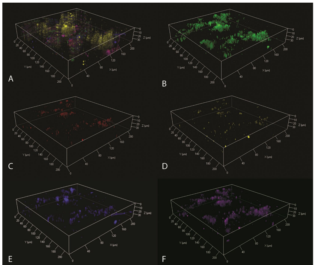
Figure 4. CLSM imaging of pH 9.5 C-13 simulant biofilm. Composite images of all stained components (A), comprising β-1,4 and β-1,3 polysaccharides (B), α-mannopyranosyl/α-glucopyranosyl sugars (C), lipids (D), proteins (E) and extracellular DNA (F).
