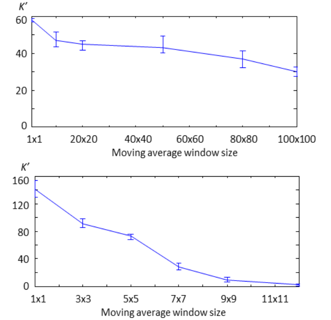
Fig. 10. Number of informative image blocks versus average window size for hand vein (top) and fingerprint (bottom)
