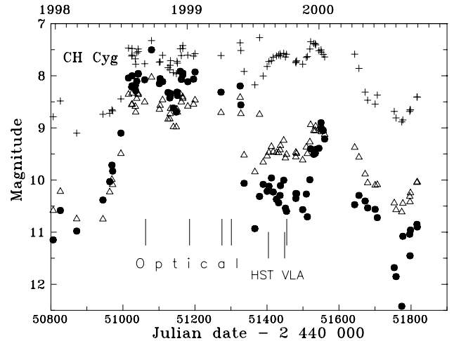
Figure 2. The U (●), B (Δ), V (+) lightcurves of CH Cyg covering its recent (1998–2000) active phase. The minimum observed between the end of 1999 and 2000 January was caused by the eclipse of the active star in the symbiotic pair by the giant on the outer, 14.5-yr period, orbit. The last observations made in 2000 April suggest a fading of activity. The vertical bars mark the times of our spectroscopic, HST and VLA observations.
