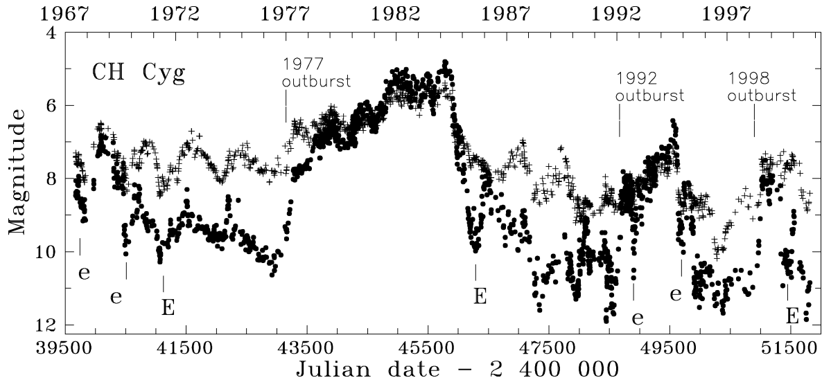
Figure 1. The U(\bullet) and V(+) lightcurves of CH Cyg during its symbiotic phase. Periods of activity are seen best in U . Eclipses in the outer and the inner binary are denoted by E and e, respectively.
