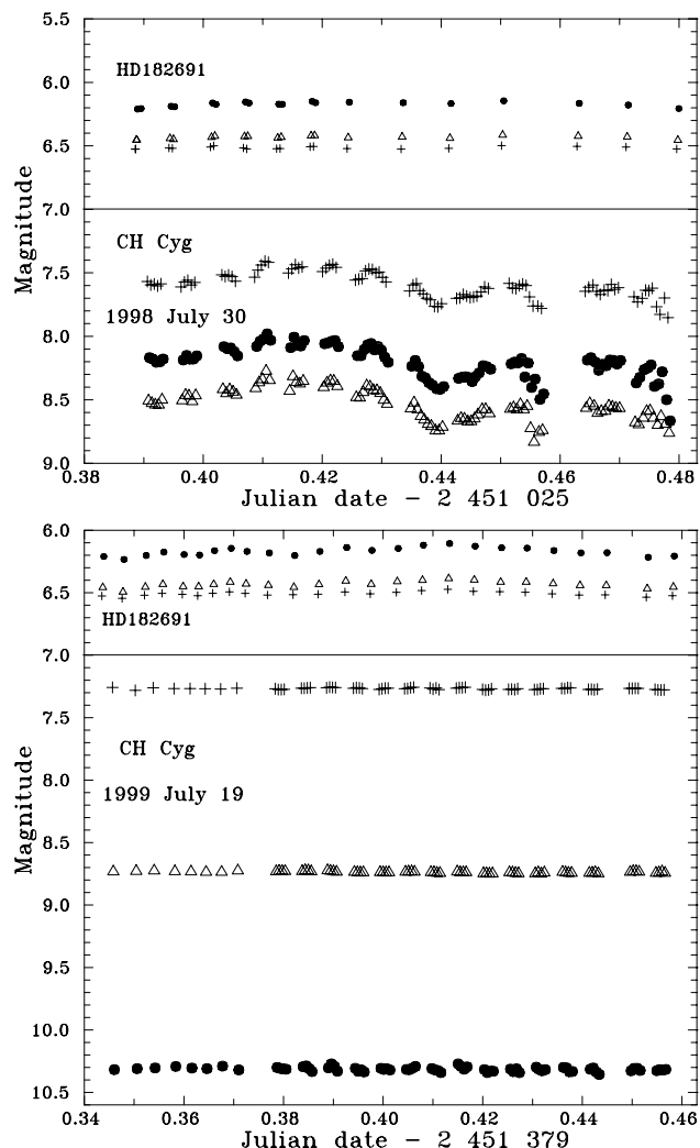
Figure 3. Example of a short-term variation during two nights located out of (1998 July 30) and in (1999 July 19) eclipse. Observations are U(●), B(Δ), V(+) magnitudes respectively.
