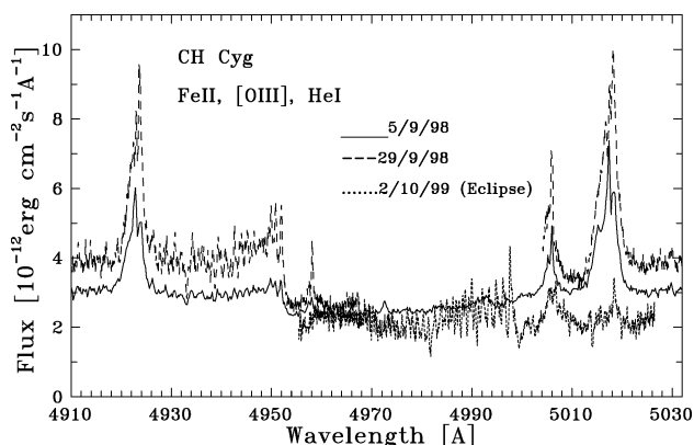
Figure 8. Development of the nebular [O III] 5007-Å line is connected with the extended nebula surrounding CH Cyg. The line is seen well also during eclipse. Note that the He I 5016-Å line is subject to eclipse.
