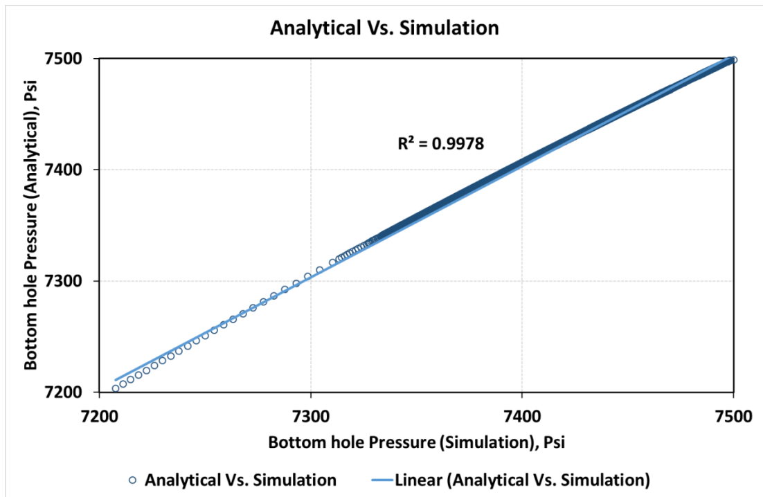
Figure 3 Predicated bottom hole pressure by the analytical model (Equation 2) vs the simulation model.
