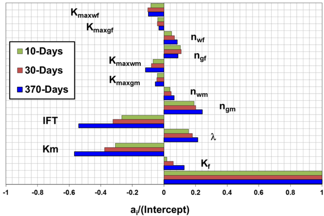
Figure 11 Tornado chart comparing LRSM coefficients of all pertinent parameters at three production stages for the Layer 2, Bottom Layer of set 45.
