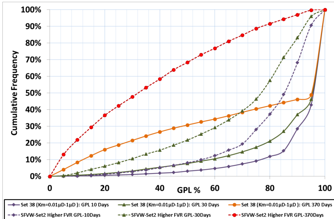
Figure 19 Histogram chart comparing the cumulative frequency of Set 38 with FVR=10, K_{\text{mr}}=100 and ST=20 and Set 2 with FVR=10 at three production periods.
