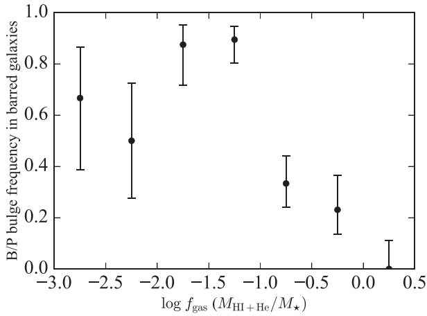
Figure 6. Frequency of B/P bulges within bars as a function of gas mass ratio f_{\text{gas}} (= M_{\text{HI}+\text{He}}/M_*) .
