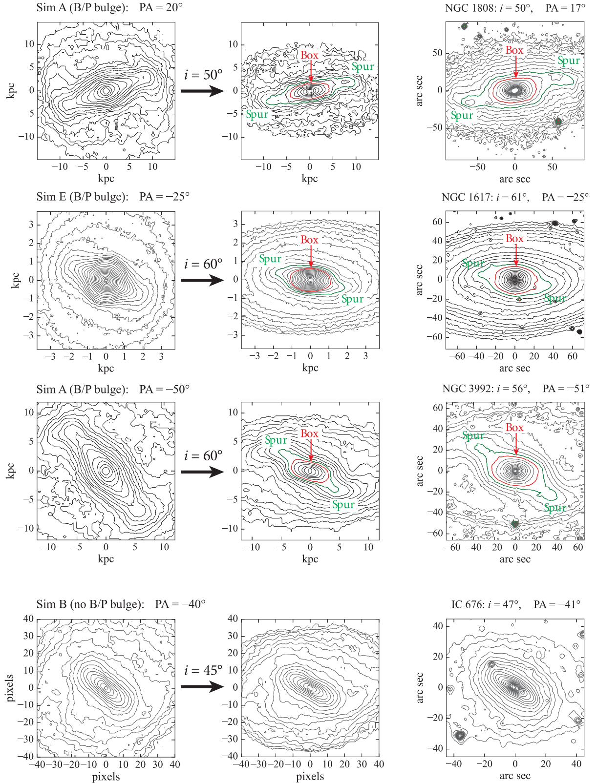
Figure 3. Projection effects on isophotes for bars with and without B/P bulges. Upper three rows: left-hand panels show face-on views of barred-galaxy simulations with B/P bulges, with bars rotated at specified angles \Delta PA_{\text{bar}} with respect to line of nodes (horizontal); middle panels show same simulation projected at indicated inclinations. Right-hand panels show real galaxies (S 4 G 3.6 \mu\text{m} images, except H band from Eskridge et al. 2002 for NGC 1808) with similar orientations (rotated so disc major axes are horizontal). Approximate regions of the ‘box’ (boxy or oval projection of the B/P bulge) are outlined in red and the ‘spurs’ (projection of the outer, vertically thin part of the bar) are outlined in green (see Erwin & Debattista 2013 for more examples). Bottom row: left: face-on view of simulation with vertically thin bar (no B/P bulge). Middle: same simulation at i = 45^\circ . Right: SB0 galaxy IC 676 (S 4 G image). Note that these bars show symmetric, elliptical isophotes, with no box+spurs morphology, due to the absence of a B/P bulge (see Appendix H for details of the simulations).
