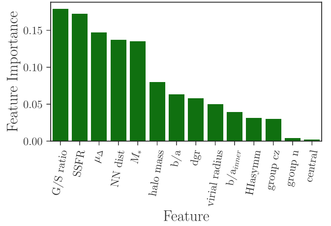
Figure 6. Relative importance of each feature input into our Random Forest classifier in predicting whether a galaxy has a tidal feature. The top five most important parameters are: G/S, SSFR, \mu_\Delta , nearest neighbor distance, and stellar mass. The others correspond to, in decreasing order, group halo mass, axial ratio b/a , (g-r) color gradient, group virial radius, axial ratio of the inner disk region of the galaxy, H I asymmetry, group redshift, number of group members, and central status (1 or 0).
