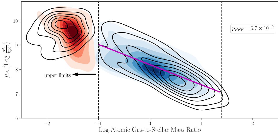
Figure 10. Distributions of \mu_{\Delta} vs. G/S for TF (black contours) and NTF (blue/red contours) galaxies. The gas-rich galaxies (including those estimated using the photometric gas fractions technique; see Section 2.1.3) are shown in blue, while the gas-poor galaxies are shown in red. For each subsample, the lowest contour contains at least 95% of the data. The linear fit of \mu_{\Delta} vs. \log(\text{G/S}) for gas-poor galaxies is shown in purple. The dashed lines mark the region over which the best-fit line is calculated, corresponding to regions where the vertical scatter from the line appears symmetrical. Gas-rich TF galaxies are more concentrated to higher G/S and lower \mu_{\Delta} , appearing more diskier, with the difference from the distribution for NTF galaxies at a p_{\text{PFF}} \sim 10^{-9} significance.
