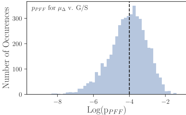
Figure 24. Distribution of the p_{\text{PFF}} comparing TF and NTF \mu_{\Delta} vs. G/S distributions for 5000 mock TF and NTF samples based on merger rates and visibility timescales as a function of gas fraction. The median p_{\text{PFF}} value is \sim 10^{-4} , marked by a vertical dashed line.
