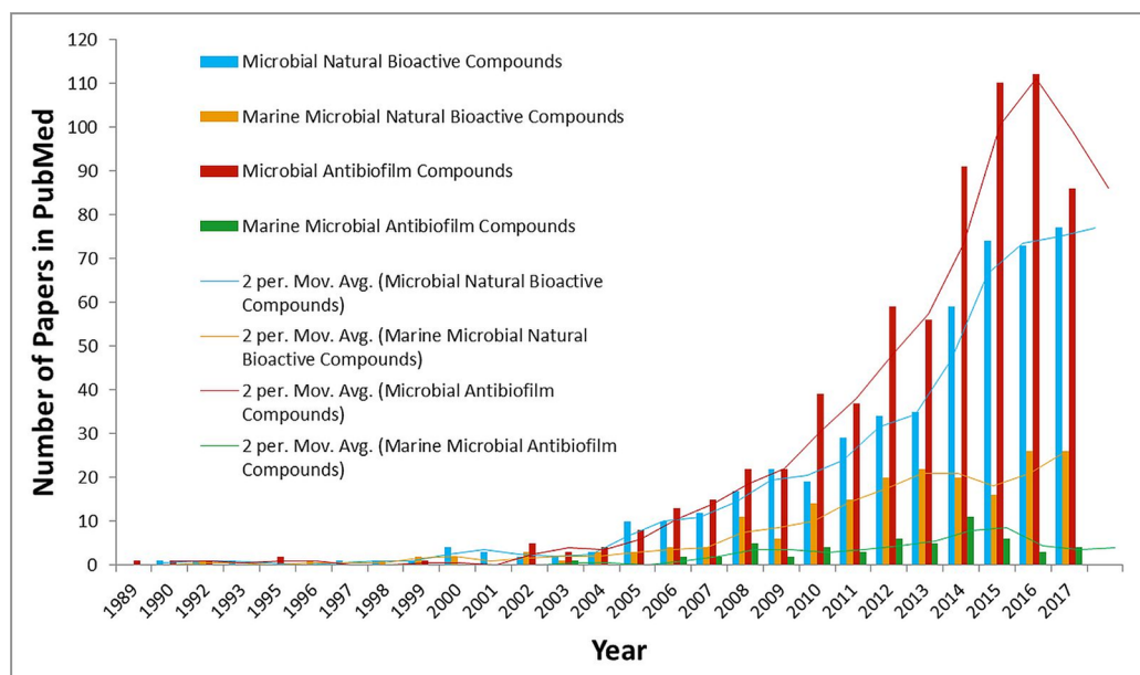
Figure 1 Comparative statistical data about number of publications in PubMed since 1989 till 2017. Comparative general data about the number of publications in PubMed when searching for several keywords/phrases: (1) microbial natural bioactive compounds (blue column); (2) marine microbial natural bioactive compounds (yellow column); (3) microbial anti-biofilm compounds (red column); and (4) marine microbial anti-biofilm compounds (green column). Moving average trend lines show the importance and urgent need for research concerning on marine microbial natural anti-biofouling/anti-biofilm compounds. Full-size DOI: 10.7717/peerj.5049/fig-1
