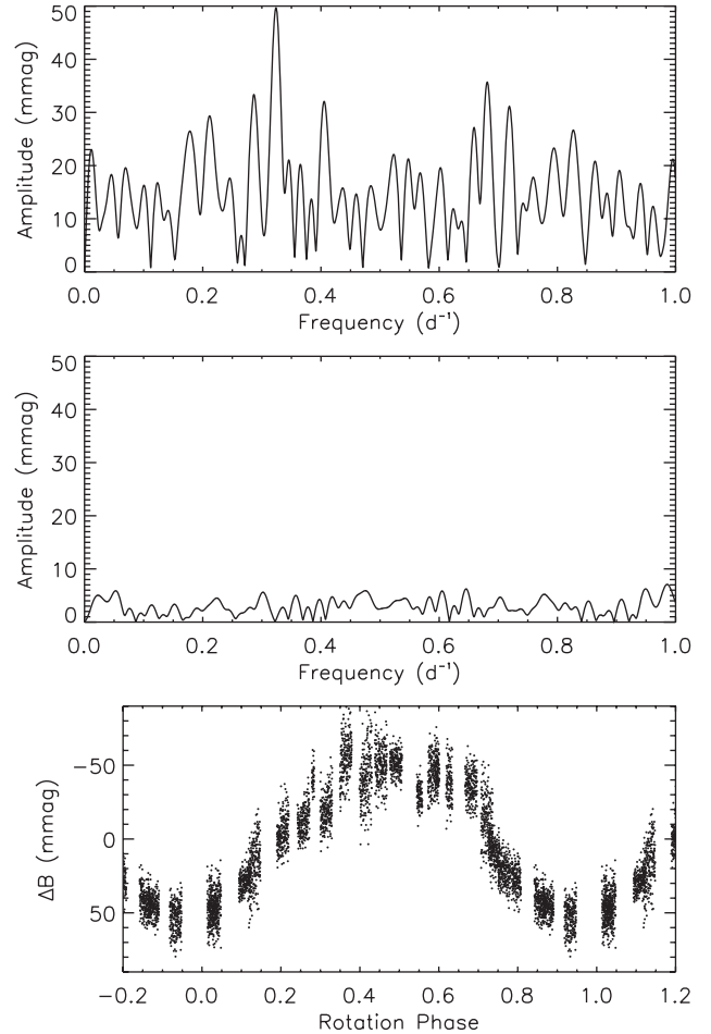
Figure 1. Top: low-frequency amplitude spectrum of J0855 showing the rotation frequency of the star at 0.32344 \pm 0.00017 \text{ d}^{-1} . Middle: amplitude spectrum of the residuals after pre-whitening the rotation signal from the data, showing the significance of the rotation peak in the top panel. Bottom: light curve folded on the rotation period of the star.
