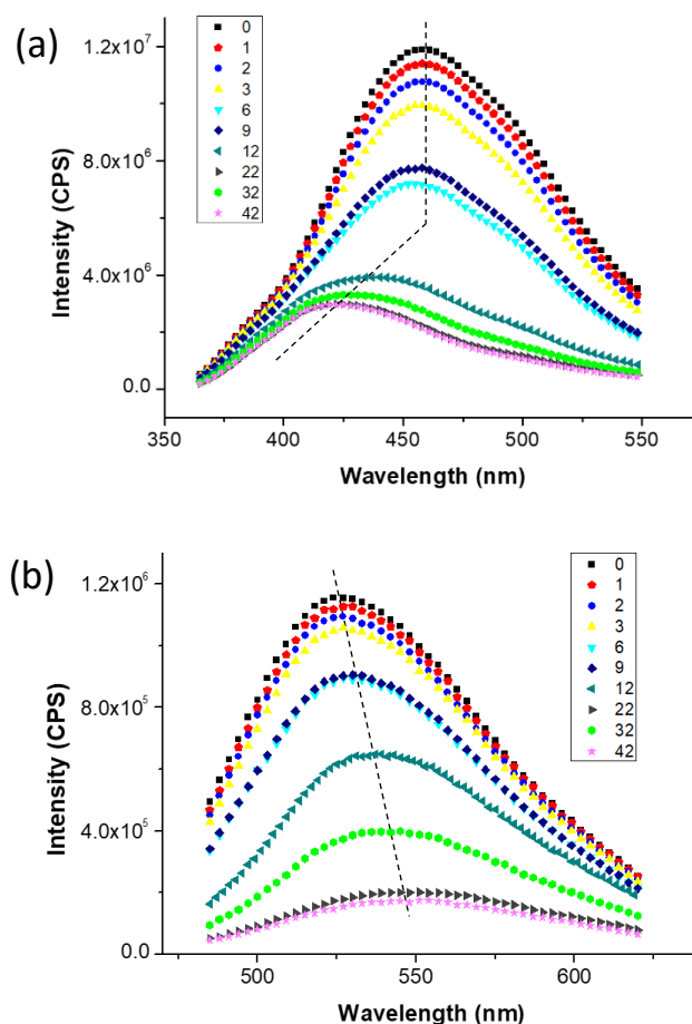
Figure 4. PL emission spectra of 10 \mu g/ml aqueous dispersions of C-dots that have been subjected to 0,1,2,3,6,9,12,22,32,42 cyclic voltammetry cycles at excitation wavelengths: (a) 380 nm and (b) 470 nm. The black dotted lines are guide to the eye.
