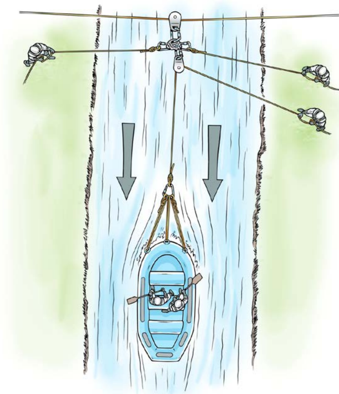
Figure 1. Boat on a Highline. Image by George Manley, courtesy of Rescue 3 (Europe). For clarity, the mechanical advantage rigging of the highline and reeving lines have been omitted.
