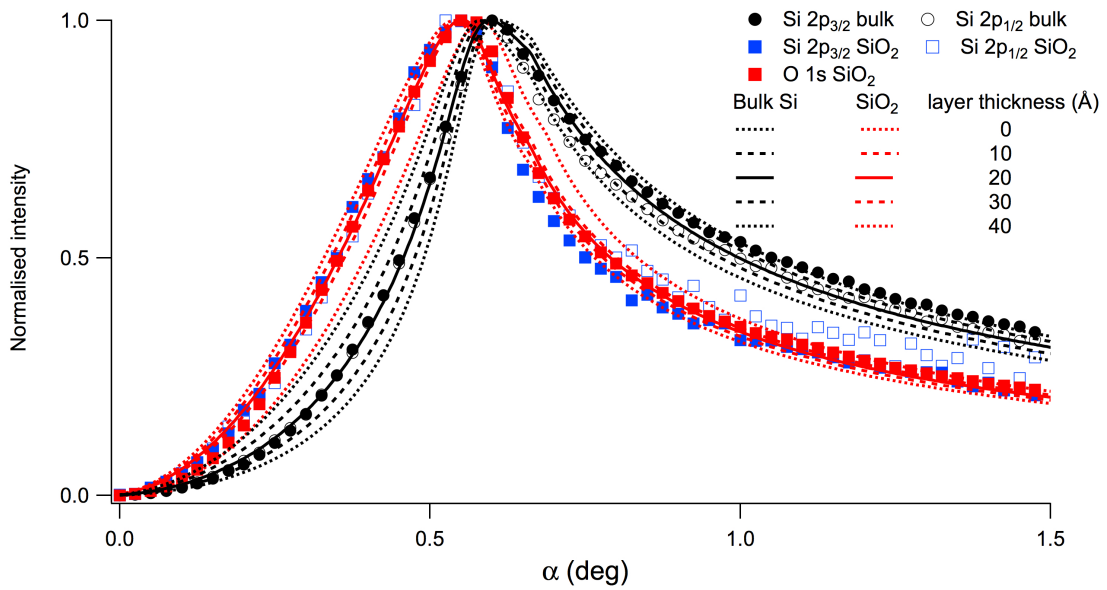
Figure A1. VPXSW scans of the O 1s, Si 2p 1/2 and Si 2p 3/2 for Si bulk and SiO 2 . The simulations for bulk and oxide layer (normalised to 1 and corrected for footprint and path length) are for an oxide layer thicknesses of 0, 10, 20, 30 and 40 Å thick, see cartoon in Fig. 6 of paper.
