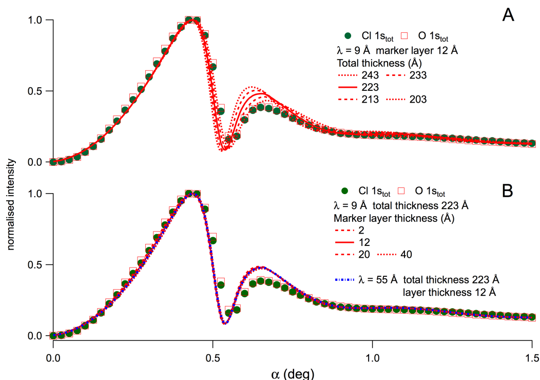
Figure A2. A, Cl 1s_{tot} and O 1s_{tot} VPXSW data with simulations using a 12 Å thick marker layer and total thicknesses of 203, 213, 223, 233 and 243 Å. B, Cl 1s_{tot} and O 1s_{tot} VPXSW data with simulations using a total thickness of 223 Å and marker layer thicknesses of 2, 12, 20, and 40 Å. All simulations used \lambda = 9 Å except for one plot in B which used \lambda = 55 Å. All simulations are footprint and path length corrected and have been shifted by 0.025^\circ .
