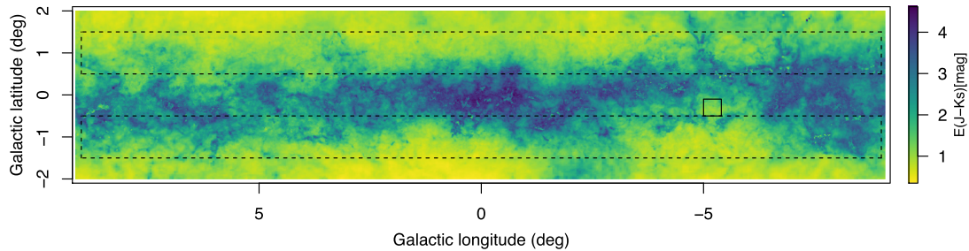
Figure 1. Reddening map of the in-plane regions of the MW, with a 1' spatial resolution, for Galactic longitudes -10^\circ < l < +10^\circ and latitudes -2^\circ < b < +2^\circ . Dashed boxes mark the regions analysed in this work. A particularly low extinction window is also marked as a solid line box. The complete map, including the outer regions presented in Gonzalez et al. (2012), is available via an interpolation code from http://mill.astro.puc.cl/BEAM .
