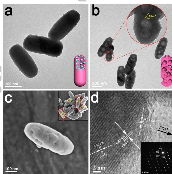
Figure 1. TEM images of PS- \text{TiO}_2 and porous \text{TiO}_2 (a, b), FESEM image of porous \text{TiO}_2 (c), HRTEM and SAD images (inset) of porous \text{TiO}_2 (d).
