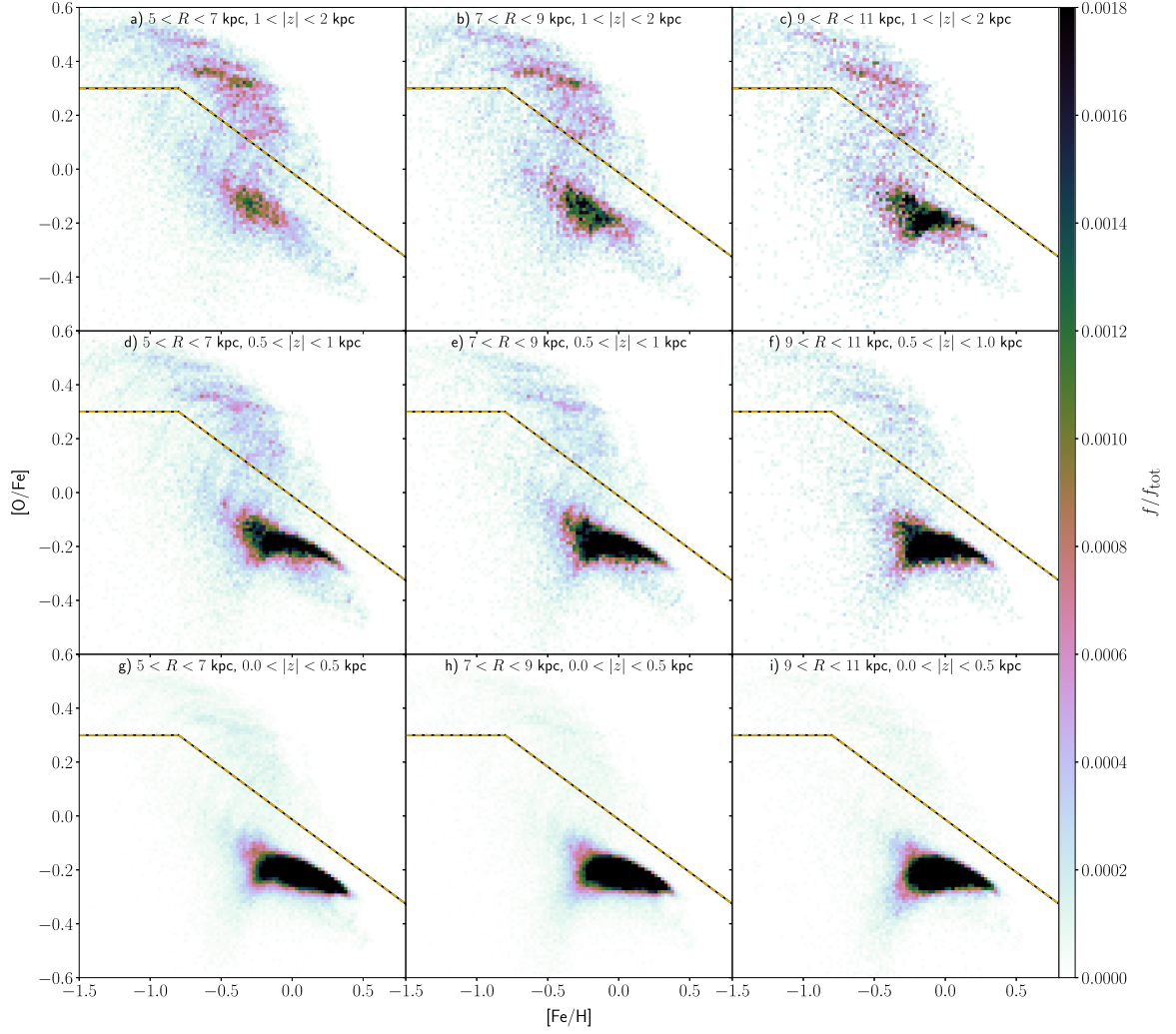
Figure 3. [O/Fe] - [Fe/H] distributions of the simulation for various radial and height cuts, as labelled in each panel. The dashed yellow–black line, defined by equation (1), separates the the high- \alpha and low- \alpha sequences. Each panel is normalized to a total weight of unity.
