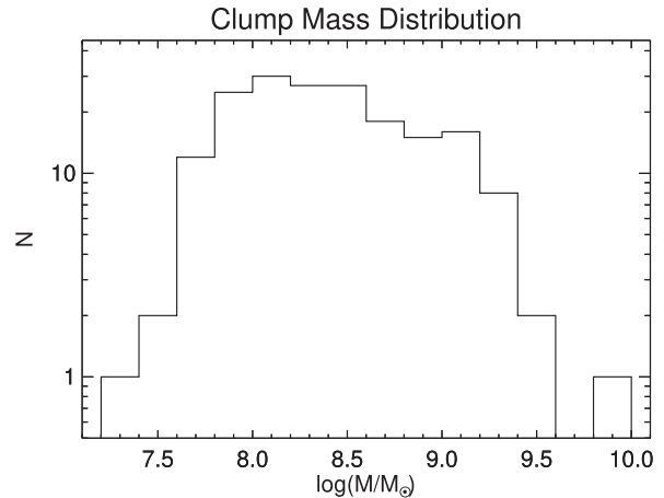
Figure 18. The distribution of clump masses which ranges from \sim 3 \times 10^7 to 10^{10} \text{ M}_{\odot} .
