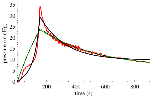
Figure 3. The pressure as a function of time in a murine bladder (red) and predicted via neo-Hookean QLV (green), Fung QLV (black, solid) and linear viscoelasticity (black, dashed).
