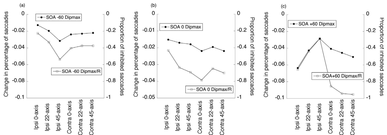
Figure 1. (a)–(c). Comparison of the change in the percentage of saccades ( \text{Dip}_{\max} = distractor – baseline) and ratio ( \text{Dip}_{\max}/R = distractor – baseline/baseline) measures of SI using data from Walker and Benson experiment 2 for: (a) –60 ms SOA, (b) 0 ms SOA, (c) +60 ms SOA. It can be seen that the two measures of SI are broadly comparable across distractor spatial location and SOA. The one case where the ratio measure departs from the percentage change is for the delayed onset (+60 ms) condition and it remains to be seen if this difference between the measures is a robust finding.
