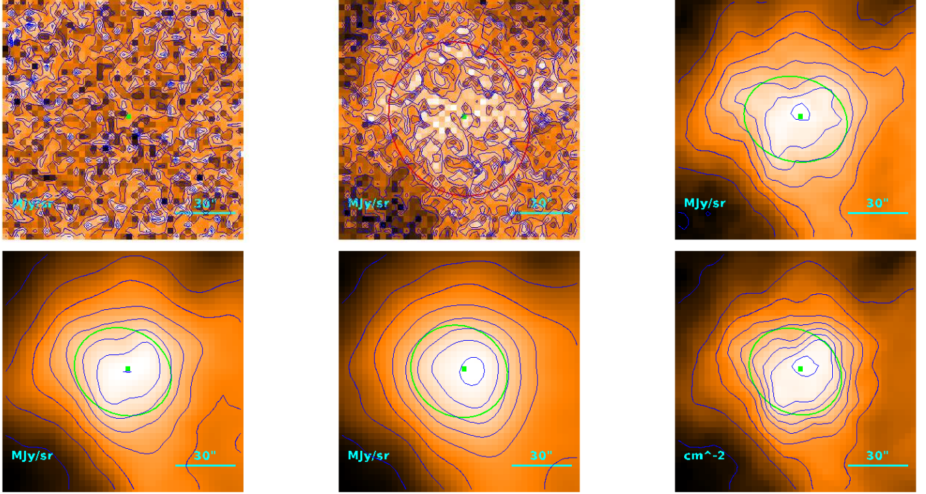
Fig. A.2. Same as Fig. A.1 for the HGBS-J154024.0-33373 dense core of our catalogue that has been classified as a prestellar core. Red ellipse indicates an uncertain flux estimate (see text for details).
