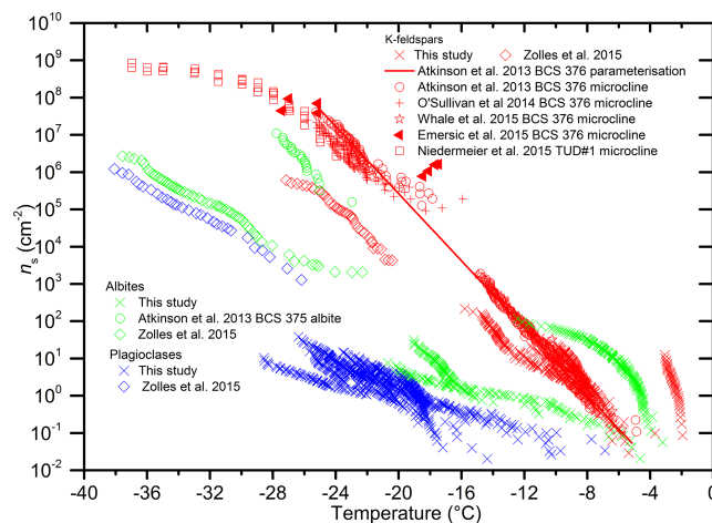
Figure 5. Comparison of literature data from Atkinson et al. (2013), Emersic et al. (2015), Niedermeier et al. (2015) and Zolles et al. (2015) with data from this study. Feldspars are coloured according to their composition, as in Fig. 3. 0.1 wt % data for Amelia albite and LD1 microcline, which is not shown in Fig. 3, has been included. Where samples are known to lose activity with time the most active runs have been shown. Note that data from Niedermeier et al. (2015) include some data from Augustin-Bauditz et al. (2014).
