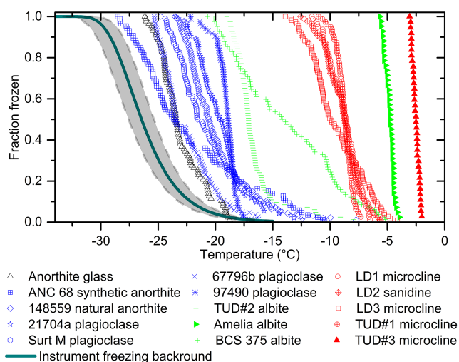
Figure 2. Droplet fraction frozen as a function of temperature for 1 wt % suspensions of ground powders of various feldspar samples. The K-feldspars are coloured red, the plagioclase feldspars are coloured blue, the albites are coloured green and the feldspar glass is coloured black. A fit to the background freezing of pure MilliQ water in the \mu l-NIPI instrument used by Umo et al. (2015) is also included. The shaded area around this fit shows 95 % confidence intervals for the fit. It can be seen that all the feldspar samples tested nucleate ice more efficiently than the background freezing of the instrument.
