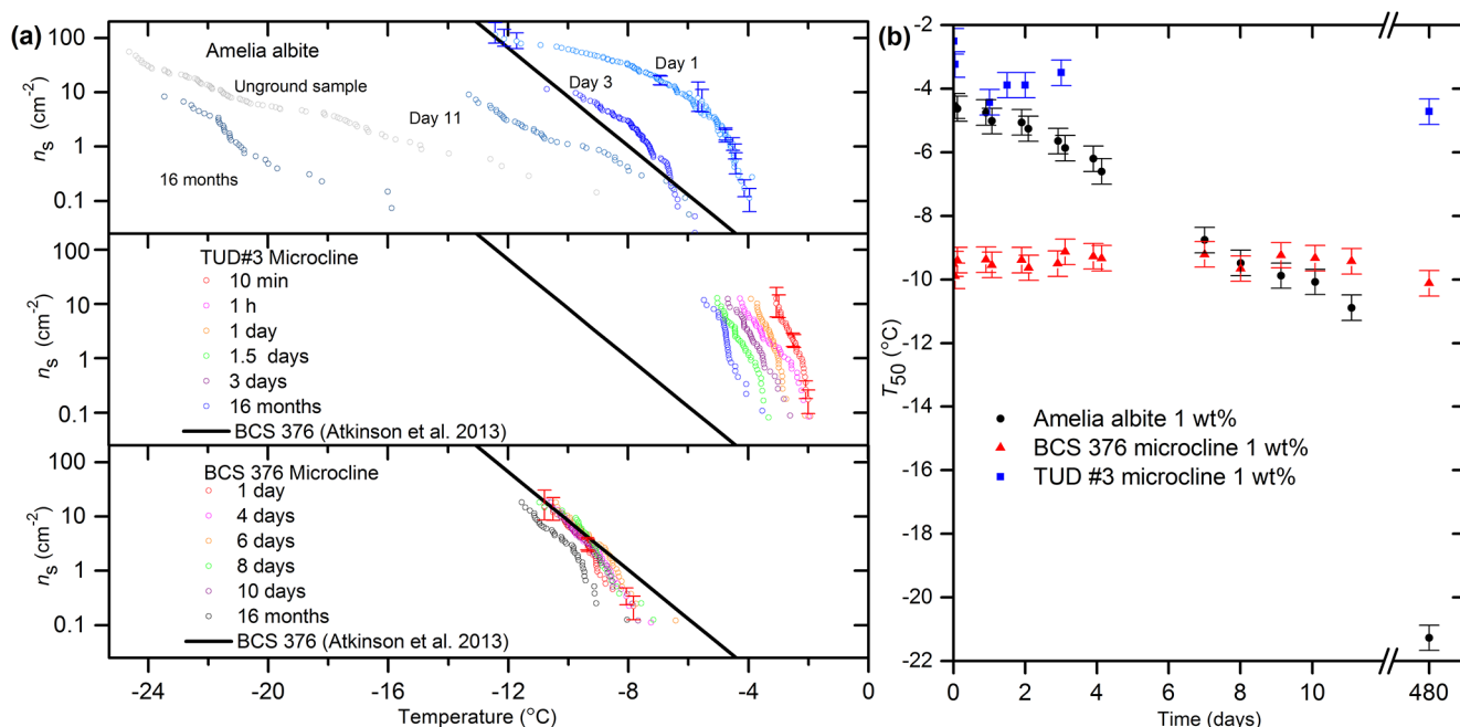
Figure 4. (a) The dependence of n_s on time spent in water for three feldspar samples. The time periods indicate how long samples were left in contact with water. Fresh samples were tested minutes after preparation of suspensions. Note that ice nucleation temperatures of BCS 376 are almost the same after 16 months in water while those of Amelia albite decreases by around 16 °C. TUD #3 microcline loses activity quickly in the first couple of days of exposure to water but total decrease in nucleation temperatures after 16 months is only around 2 °C. (b) Median freezing temperature against time left in suspension for BCS 376 microcline, TUD#3 microcline and Amelia albite. For clarity, not all curves represented by points in panel (b) are included in panel (a).
