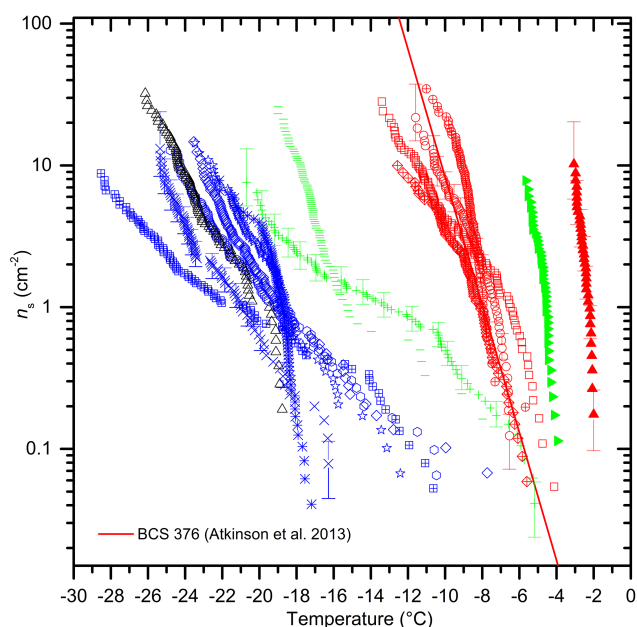
Figure 3. Ice nucleation efficiency expressed as n_s(T) for the various feldspars tested in this study. The symbols are the same as those used for Fig. 2. The K-feldspars are coloured red, the plagioclase feldspars are coloured blue, the albites are coloured green and the feldspar glass is coloured black. Except for Amelia albite and TUD#1 microcline all samples were tested twice and the data from the two runs combined. Sample information can be found in Tables 1 and 2. Temperature uncertainty is \pm 0.4 °C. Y-Error bars calculated using the Poisson Monte Carlo procedure described in Sect. 4. Data points with large uncertainties greater than an order of magnitude have been removed, these are invariably the first one or two freezing events of a given experiment. For clarity error bars have only been included on a selection of data sets (TUD#3 microcline, LD1 microcline, BCS 375 albite and 67796b plagioclase). The error bars shown are typical.
