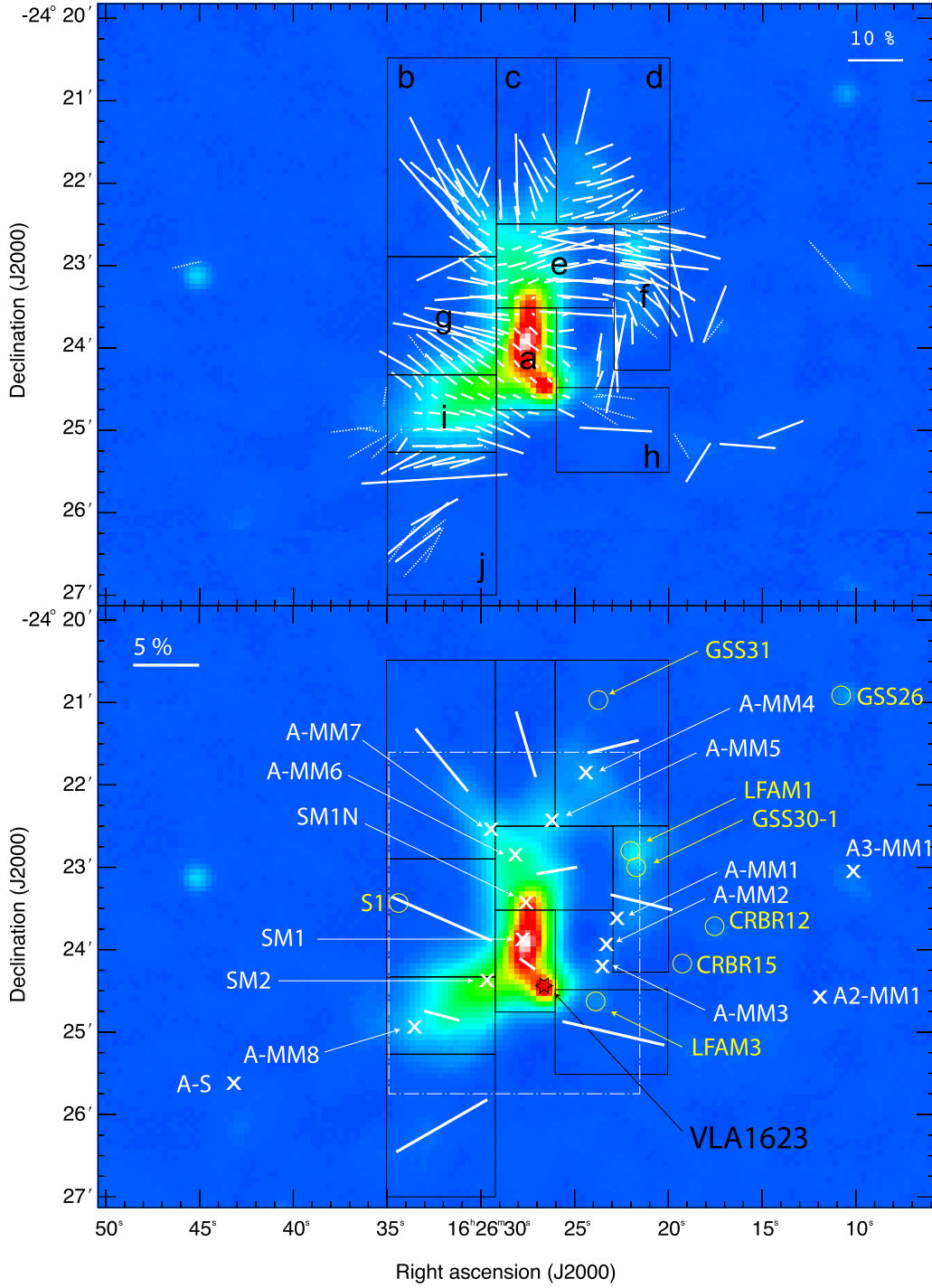
Figure 8. Close-up of the \rho Oph-A core region in Figure 1, with regions divided according to the magnetic field direction (top panel) and showing the median of the magnetic field directions of each region shown in Table 2 (bottom panel). Black boxes indicate components a–j (see Section 5.1), and 10% and 5% scale vectors are shown in the upper right (top panel) and left (bottom panel) corners, respectively. Note that P/\delta P > 2 (dotted vectors) and P/\delta P > 3 (solid vectors) data are shown here; therefore, the errors of the polarization vector angle are typically much less than 15^\circ . The region indicated with the white dashed-dotted box in the bottom panel corresponds to the region shown in Figure 10.
