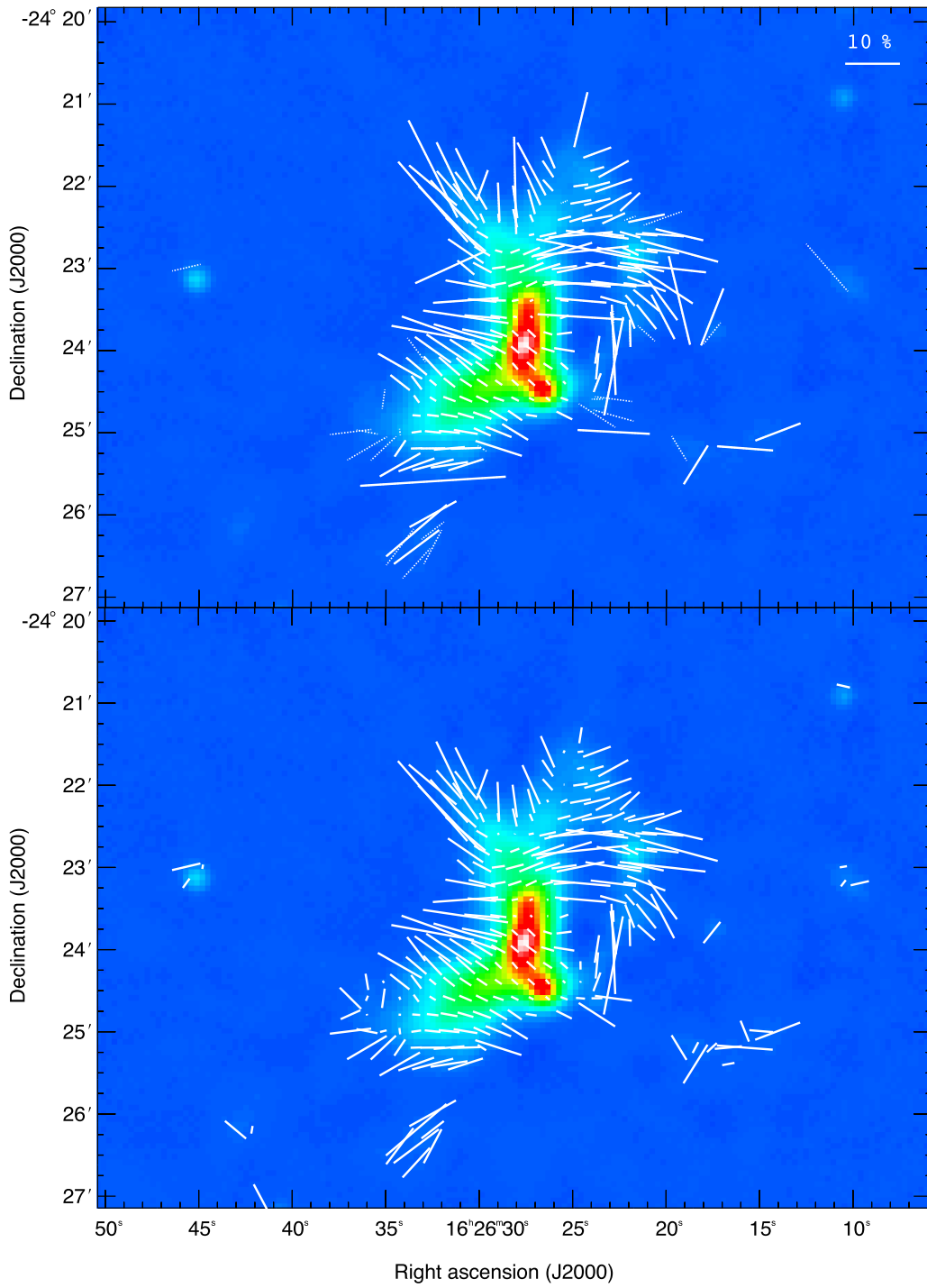
Figure 6. The 850 \mu\text{m} polarization vector maps sampled on a 12'' grid and rotated by 90^\circ (i.e., as in Figure 3 but rotated by 90^\circ ). The 90^\circ rotated vectors, which show the inferred magnetic field orientation projected on the plane of the sky, are plotted where I > 0 , P/\delta P > 2 , and \delta P < 4\% (dotted vectors) and I > 0 , P/\delta P > 3 , and \delta P < 4\% (solid vectors) in the top panel and where I > 0 and I/\delta I > 20 in the bottom panel. A 10% scale vector is shown in the upper right corner. See the text for these two panels with different selections ( P/\delta P and I/\delta I ).
