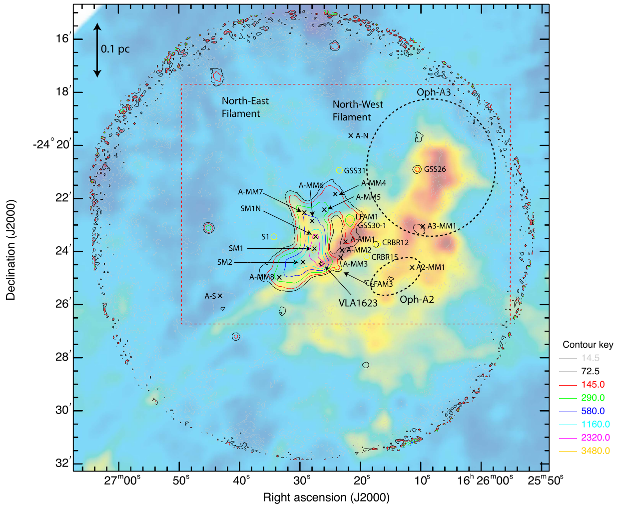
Figure 9. Contours of the 850 \mu\text{m} total intensity (Stokes I ) image (cf. Figure 1 of this work) of the \rho Oph-A field superimposed on HARP CO J = 3-2 observations showing the integrated emission between -5 and +12 \text{ km s}^{-1} (cf. Figure 1 of White et al. 2015).
