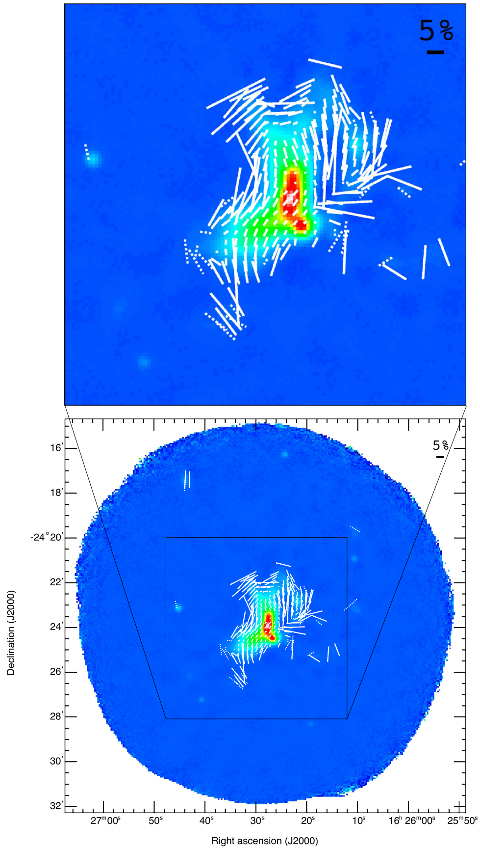
Figure 3. The 850 \mu\text{m} polarization vector maps. The vectors are sampled on a 12'' grid ( 3 \times 3 pixel smoothing) and plotted where I > 0 , P/\delta P > 2 , and \delta P < 4\% (dotted vectors) and I > 0 , P/\delta P > 3 , and \delta P < 4\% (solid vectors).
