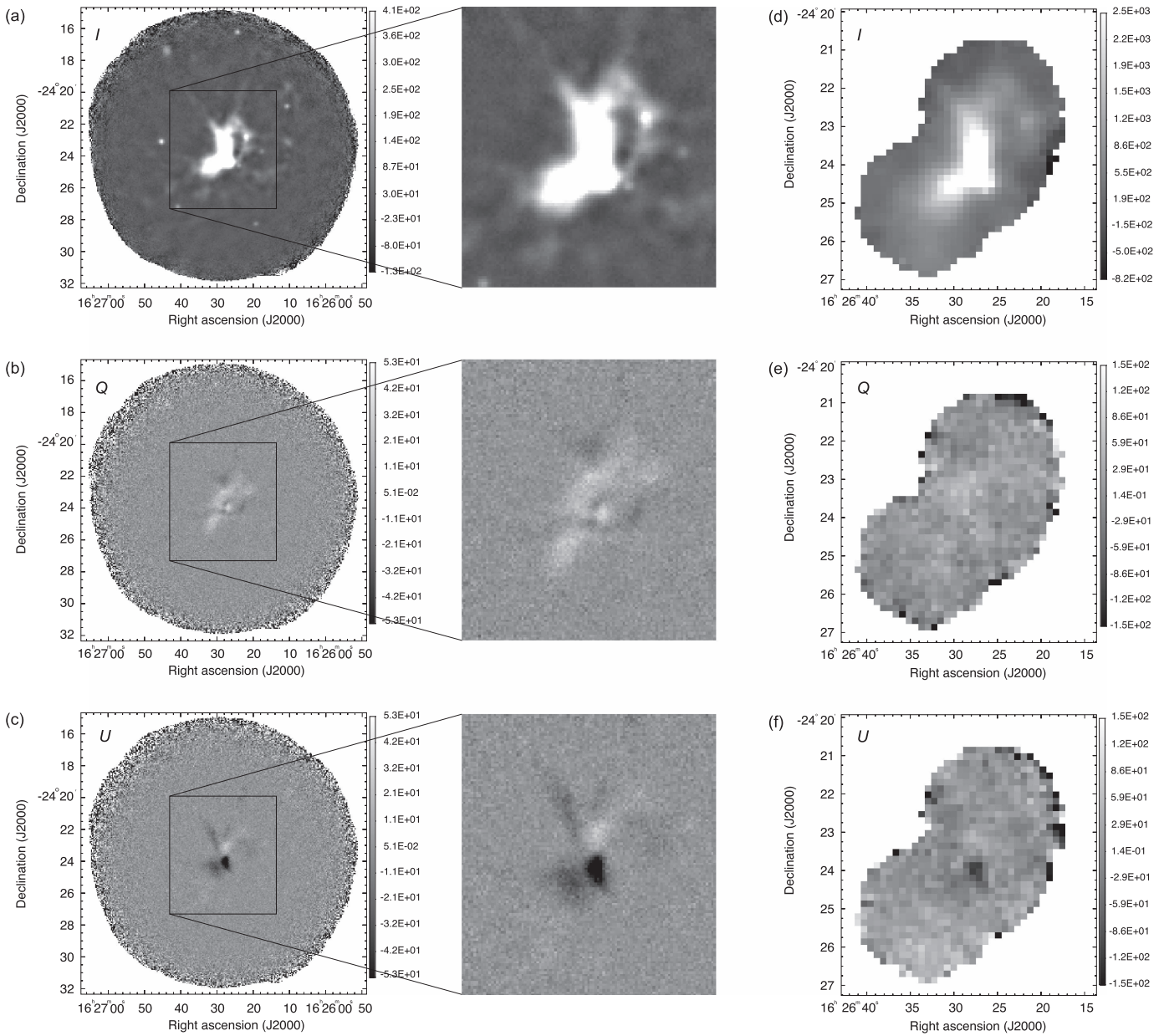
Figure 2. SCUBA-2/POL-2 data (this work) compared with SCUPOL (previous work). The intensity gray scales are different between the POL-2 and SCUPOL data. (a)–(c) Stokes I , Q , and U images (linear scale) of the \rho Oph-A core region obtained with the JCMT with SCUBA-2/POL-2. The Stokes Q and U images ((b) and (c)) have the same gray scale in units of \text{mJy beam}^{-1} . The SCUPOL field of view ((d)–(f)) is indicated by a black box in Figures 2(a)–(c), respectively. (d)–(f) 850\ \mu\text{m} Stokes I , Q , and U images of the \rho Oph-A core region obtained from the JCMT with SCUPOL (from the SCUBA Polarimeter Legacy Catalogue). The Stokes Q and U images ((e) and (f)) have the same gray scale in units of \text{mJy beam}^{-1} . The original units are \text{pW} and \text{V} in the SCUBA-2/POL-2 and SCUPOL data, which are converted to \text{mJy} using the conversion factors of 725\ \text{Jy beam}^{-1}\ \text{pW}^{-1} and 455\ \text{Jy beam}^{-1}\ \text{V}^{-1} (see Matthews et al. 2009). Note that the SCUPOL data are binned to generate 10'' vectors. The gray-scale ranges in SCUBA-2/POL-2 and SCUPOL are different so that fainter regions in the Q and U images are clearly seen in each image.
