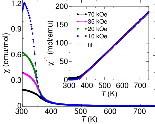
FIG. 4. (Color online) High-temperature magnetic susceptibility versus temperature measured in selected magnetic fields. Inset shows \chi^{-1}(T) , together with the fit using Eq. 1.
