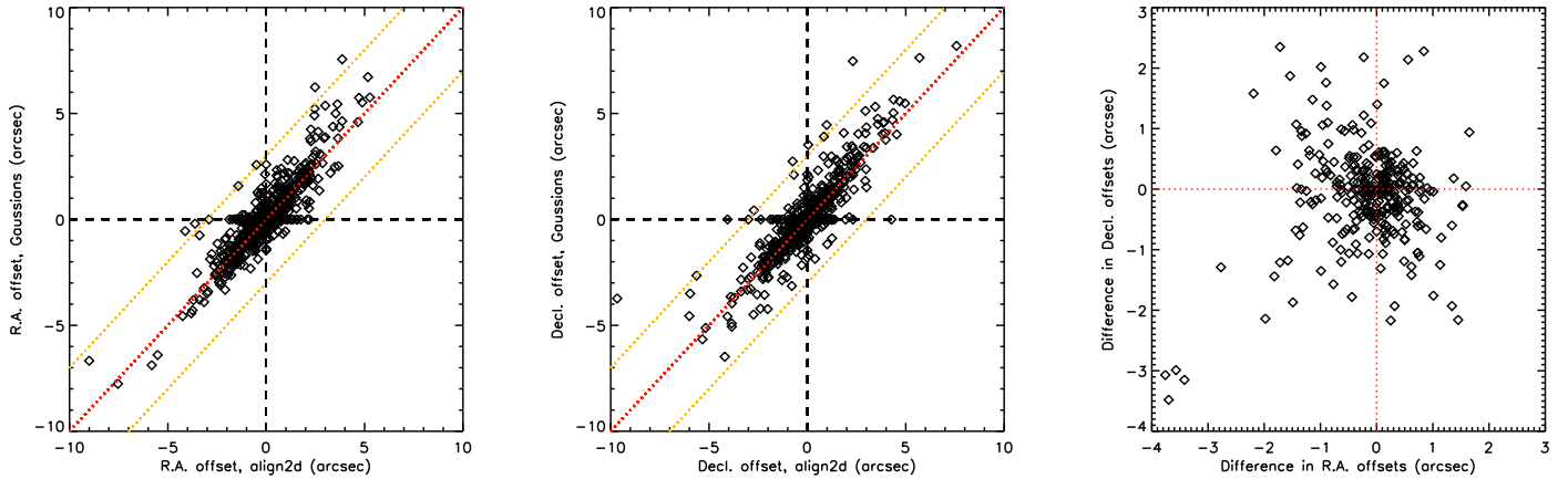
Figure 11. Offsets derived for all GBS observations using align2d and Gaussian fitting. The left and middle panels compare the offsets derived in R.A. (left) and decl. (middle) for the two methods. Here the red dotted line shows a one-to-one relationship, while the yellow dotted lines show discrepancies of 3'' (1 pixel at 850\ \mu\text{m} ) between the two measures. Offsets of zero are assigned to the relatively few observations where the method was unable to determine a measurement. The right panel shows the difference in offsets ( align2d minus Gaussian) measured in R.A. and decl. Here only observations for which offsets were measured using both methods were included.
