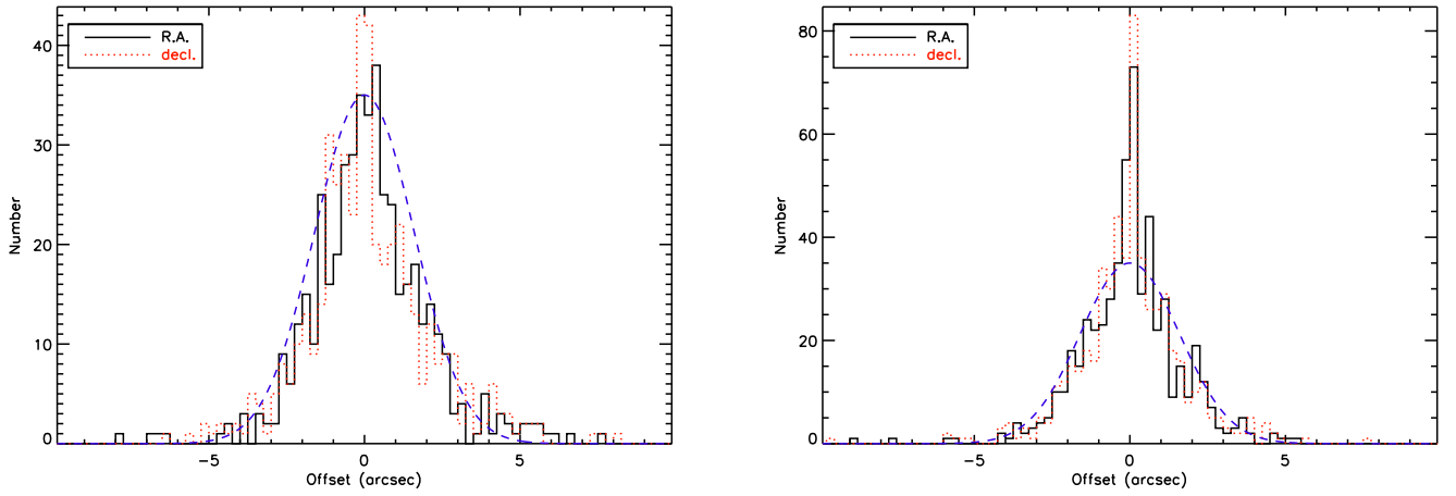
Figure 10. Pointing offsets derived for all GBS observations using the Gaussian-fit method (left) and align2d method (right). The solid black histogram shows offsets in R.A., while the dotted red histogram shows offsets in decl. Observations where the method was unable to be applied, e.g., due to insufficient flux in the map, are excluded. The blue dashed curve shows a Gaussian with \sigma = 1''.6 (left) and 1''.7 (right) for reference.
