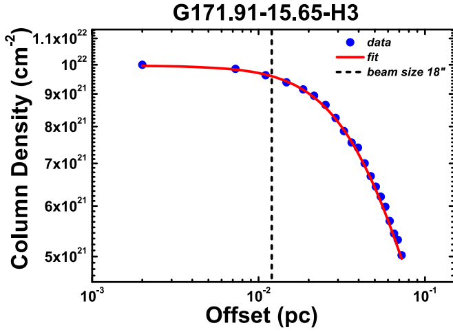
Figure 9. Column density profiles of the dense core for G171.91-15.65-H3. The red solid line represents the corresponding fit. The fitting results of N_c , R_t , and a are listed in Table 9. The flat central region and power-law decline can be seen in the figure. Due to its small size, we cannot obtain average column density distributions accurately for G170.26-16.02-H1 and G171.91-16.15-H1, and the flat region a of G171.91-15.65-H1 is smaller than the beam size. Therefore, we only present the column density profile for G171.91-15.65-H3 in this section. The images for other sources are shown in the figure set.
