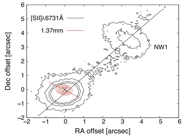
Figure 3. The 1.37 mm continuum map for M170117 (red contours) overplotted on the optical [\text{S II}]\lambda 6731 \text{ \AA} image of the HH 1165 jet (black contours). Red line is along the disc axis ( \text{PA} = 55^\circ ). Black line is along the jet axis ( \text{PA} = 320^\circ ). The contours represent the signal-to-noise levels from 2\sigma to 10\sigma in steps of 2\sigma . The 1\sigma rms is 0.8 \text{ mJy} in the 1.37 mm continuum map and 3 \times 10^{-16} \text{ erg s}^{-1} \text{ cm}^{-2} in the [\text{S II}]\lambda 6731 map. The xy -axes show the position offset relative to the 1.37 mm continuum position of M170117 (marked by a black cross). North is up, and east is to the left.
