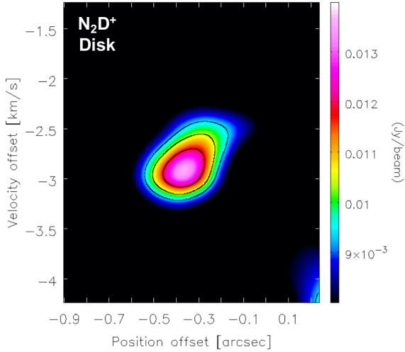
Figure 9. The PV diagrams in the N_2D^+ line emission for a cut along the disc axis. The velocity offset is with respect to the source V_{LSR} of 12.1 \text{ km s}^{-1} . The contour levels are 0.01, 0.012, 0.013, 0.014, and 0.015 \text{Jy beam}^{-1} . The base contour level is set to 0.01 \text{ Jy beam}^{-1} to enhance the peak emission positions. The blue-shifted lobe is located towards the south-west of the source.
