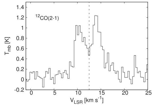
Figure 12. The ^{12}\text{CO} (2–1) spectrum for M1701117. Dashed line marks the source V_{LSR} .
