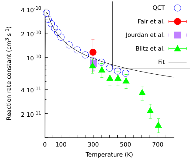
Fig. A.1. State-selected reaction rates for SO( v=0 ) + OH( v=0 ) \rightarrow SO 2 + H collisions as a function of temperature obtained in this work (QCT), and compared with the experimental results of previous works (Blitz et al. 2000; Jourdain et al. 1979; Fair & Thrush 1969). The calculated rate has been fitted to the expression K(T) = a(T/300)^b e^{-c/T} , with a = 1.24211 \times 10^{-10} \text{ cm}^3 \text{ s}^{-1} , b = -0.56049 and c = 6.58356 \text{ K} . This expression is adequate in the 10–300 K interval.
