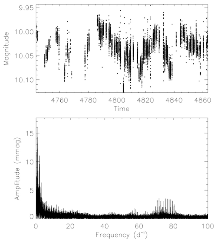
Figure 4. The variability of the known pulsating PMS star HD 34282 in the WASP data. The top panel shows the noisy light curve, with the periodogram shown in the bottom panel. The pulsations are clearly visible in the lower plot.
