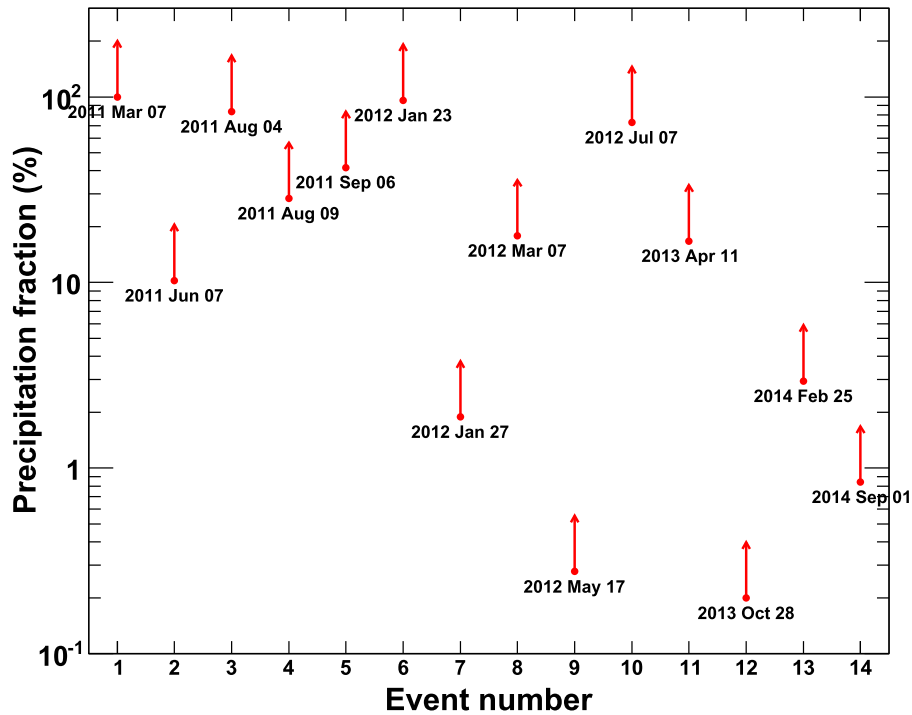
Figure 8. Lower limits on the fraction of precipitating protons N_{\text{LDGRF}}/(N_{\text{SEP}} + N_{\text{LDGRF}}) .
