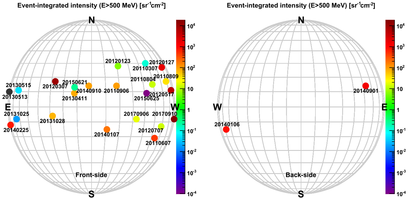
Figure 1. Heliographic locations of parent flares for the SEP events listed in Table 1. Front- and backside events are displayed in the left and right panels, respectively. The color code indicates the SEP event-integrated intensity above 500 MeV; the one event with no signal above this threshold is shown in black.
