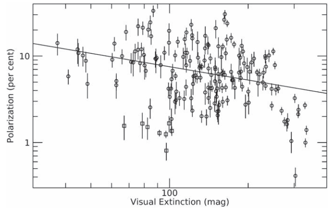
Figure 3. Relationship between the debiased polarization fraction P and the visual extinction A_V in Perseus B1. Each point represents one of the polarization vectors from the left panel of Figure 1 that also have Herschel -derived opacity measurements. The visual extinction A_V is derived from the 300\,\mu\text{m} \tau_{300} opacity map from Chen et al. (2016) assuming a reddening factor R_V = 3.1 . The figure covers a range of extinction A_V from 30 to 400 mag. The vertical lines show the uncertainties for the polarization fraction P . The eight polarization vectors found toward B1-c are identified with squares. The solid line is the power-law fit (with index \beta \sim -0.5 ) between the polarization fraction P and the visual extinction A_V ( P \propto A_V^\beta ; see Section 3.2).
