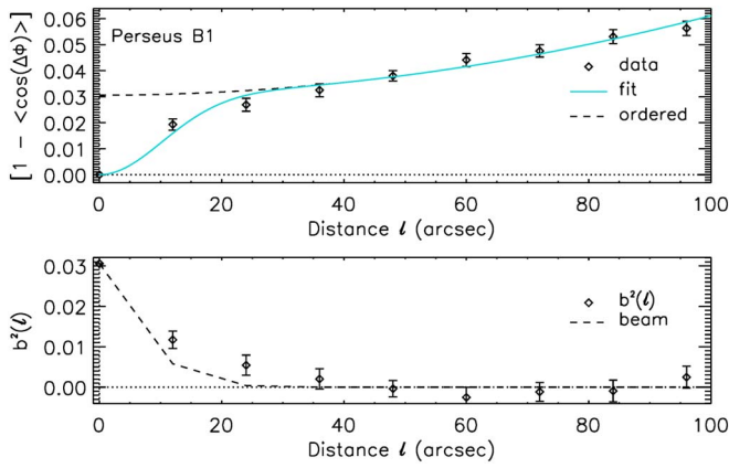
Figure 7. Dispersion of polarization angles for POL-2 observations of Perseus B1. Top: angular dispersion function [1 - \cos(\Delta\Phi)] as a function of the distance \ell . The fit of Equation (10) to the data is shown including (blue solid line) and without including (black dashed line) the autocorrelation function b^2(\ell) defined in Equation (11). Bottom: signal-integrated turbulence autocorrelation function b^2(\ell) as a function of distance \ell . The black dashed line shows the contribution of the telescope beam alone.
