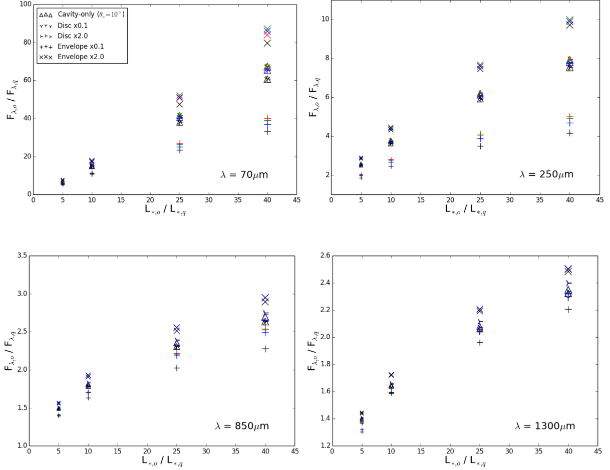
Figure 6. Outburst-to-quiescent flux ratios, F_{\lambda,o}/F_{\lambda,q} , at 70, 250, 850, and 1300 \mu\text{m} , as a function of the protostellar luminosity L_{*,o} , computed integrating over the inner R \leq 10\,000 AU. The red, green, blue, and black markers correspond to SEDs at 0^\circ , 30^\circ , 60^\circ , and 90^\circ , respectively. The triangles represent the default model (no rescaling), upward/downward tri-spoke markers are models with disc masses rescaled to 0.1/2 times the simulation values, and plus/cross markers are models with envelope masses scaled 0.1/2 times.
