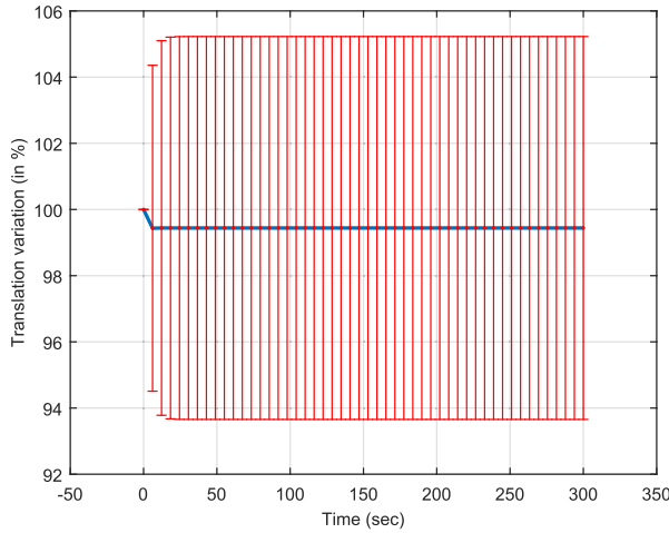
FIGURE 2. Principal behavior and robustness of the non-stress model, when the rate constants of the model undergo fluctuations upto \pm 50\% from its original value. Blue solid line represents principal behavior and red lines represent standard deviation from principal behavior when parameters are fluctuated.
