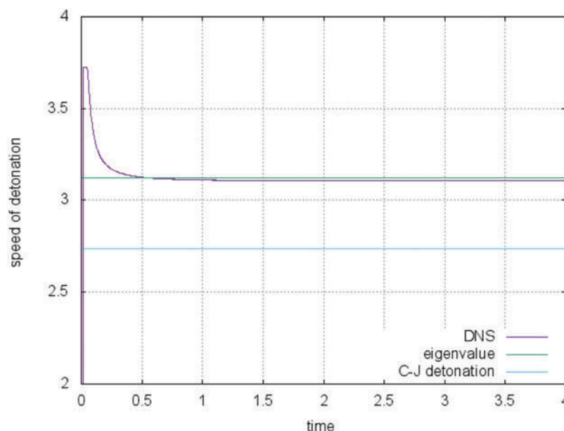
Figure 4. Comparison of the speed of detonations produced by DNS with the detonation speed predicted by the eigenvalue problem and C–J detonation speed ( q_0 = 5.0 , A = 2 \times 10^5 , E_a = 15 and \gamma = 1.32 ).
