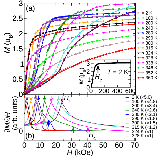
FIG. 2. (Color online) (a) Isothermal magnetization curves (per f.u.) measured at selected temperatures. The inset shows M(H) data recorded at 2 K in pulsed magnetic fields up to 600 kOe. (b) Field dependencies of \partial M/\partial H . Arrows indicate positions of peaks in the \partial M/\partial H vs H curves that are used as estimates for H_t and H_c at different temperatures.
