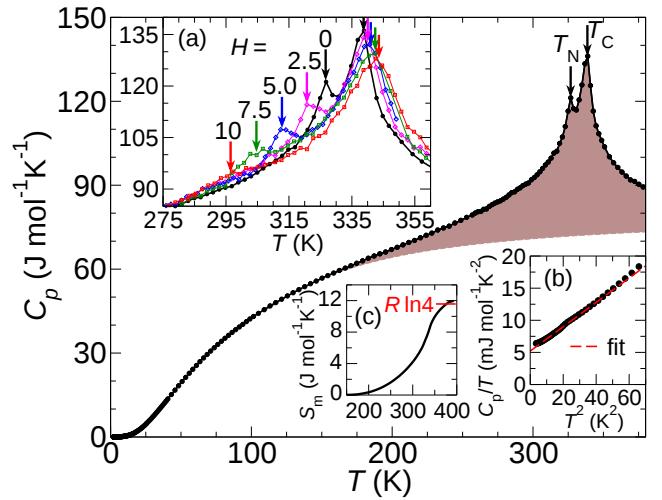
FIG. 5. (Color online) Specific heat of MnPtSi. Magnetic phase transitions are indicated. The brown area represents the magnetic specific heat estimated as described in the text. Insets: (a) Specific heat in selected external magnetic fields. The values of H (kOe) are given above the arrows indicating the transition temperatures; (b) C_p/T plotted versus T^2 . The red dashed line represents the fit to the experimental data using Eq. 2; (c) Magnetic entropy.
