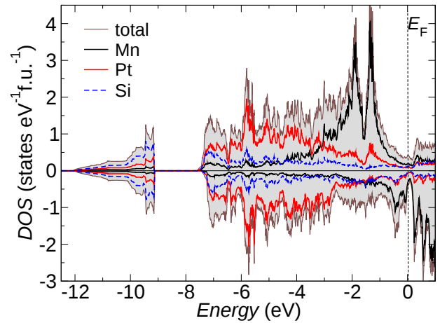
FIG. 10. (Color online) The total and atomic resolved DOSs for MnPtSi calculated assuming the FM state. The majority (minority) spin was plotted upward (downward).
