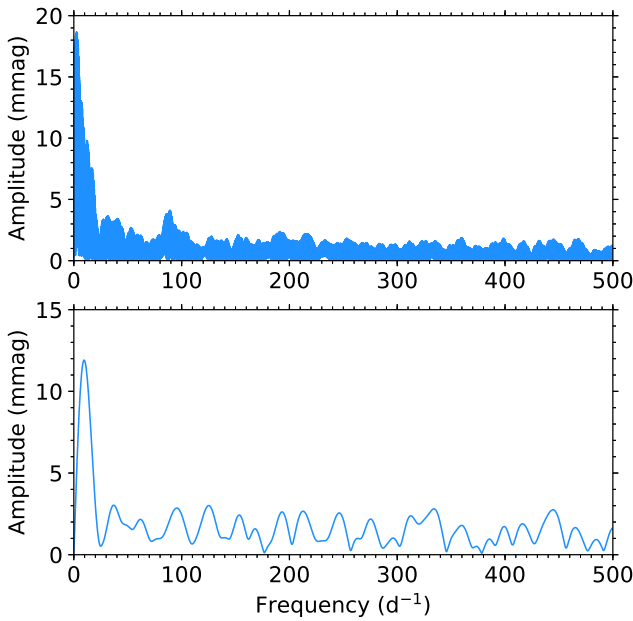
Fig. 4. Amplitude spectrum of the SAAO photometry of HD 158596 for all photometry ( top panel ) and the longest uninterrupted section ( bottom panel ).
