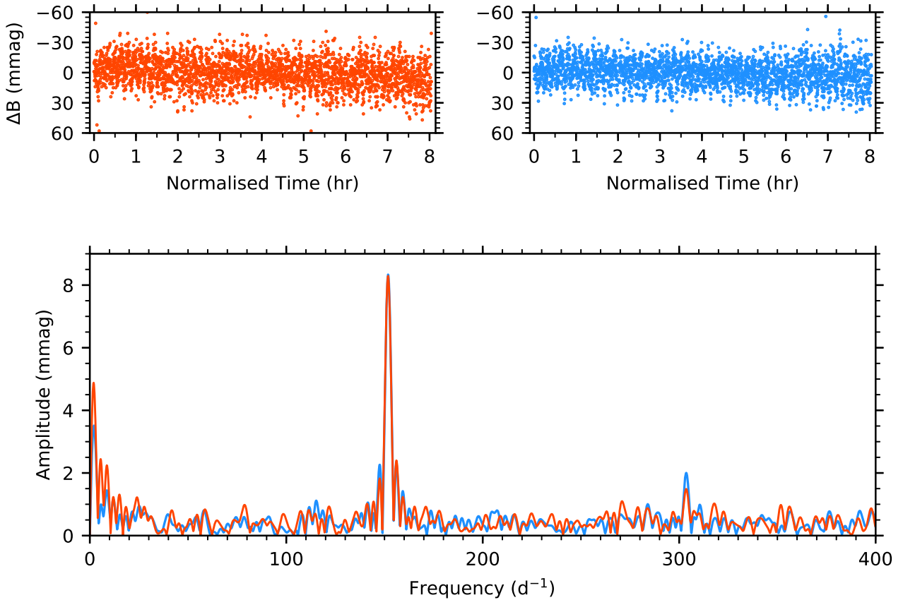
Fig. 3. Differential light curves of the roAp star J1640 extracted using the DOPHOT pipeline (red; top-left ) and with the our TEA-PHOT pipeline (blue; top-right ). These data were obtained using the SHOC instrument at SAAO on 12 June 2017. Bottom panel: difference in the S/N of the pulsation mode at 151.93 \text{ d}^{-1} and its harmonic at 303.86 \text{ d}^{-1} in the amplitude spectra of these two light curves.
