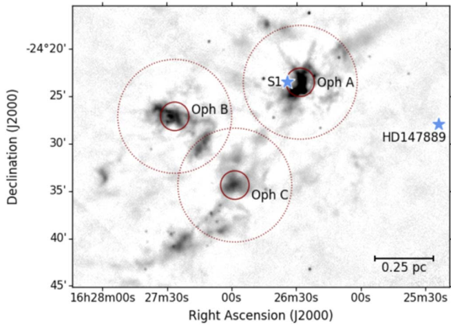
Figure 4. Finding chart for the L1688 region. The gray-scale image shows the JCMT Gould Belt Survey SCUBA-2 850 \mu\text{m} map of the region (Pattle et al. 2015). The three BISTRO fields are marked in red: solid lines show the central 3' diameter regions with uniform noise characteristics used in this work, and dotted lines show the full extent of the observations. The locations of the B stars HD 147889 and S1 are marked with blue stars. A plane-of-sky distance of 0.25 pc at our assumed distance to L1688 of 138 pc is shown in the lower right corner.
