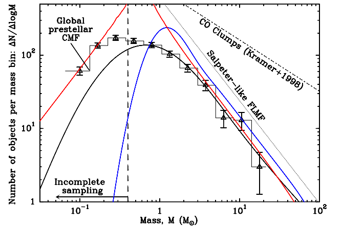
Fig. B.2. Comparison of the prestellar CMF observed in Orion B (black triangular data points and histogram from Könyves et al. 2019; see also Fig. 3) with the global prestellar CMFs expected in the toy model of Sect. 3, under three assumptions about the shape of the CMF generated by a single filament of line mass M_{\text{line}} : (i) lognormal f_{M_{\text{line}}}(m) distribution (Eq. (2)) with \sigma_{M_{\text{line}}} = \sqrt{0.4^2 + 0.3 [\log(M_{\text{BE,eff}}/M_{\text{BE,th}})]^2} (fiducial case, black curve); (ii) lognormal f_{M_{\text{line}}}(m) distribution (Eq. (2)) with fixed \sigma_{M_{\text{line}}} = 0.2 independent of M_{\text{line}} (blue curve); and (iii) broken power law, f_{M_{\text{line}}}(m) \propto m^6 for m < M_{\text{BE,th}} , f_{M_{\text{line}}}(m) = \text{constant} for M_{\text{BE,th}} \leq m < M_{\text{BE,eff}} , f_{M_{\text{line}}}(m) \propto m^{-4} for m > M_{\text{BE,eff}} (red curve). For reference, the black dotted line displays the Salpeter-like power-law FLMF, dN/d\log M_{\text{line}} \propto M_{\text{line}}^{-1.4} , observed in the supercritical line mass regime (see Fig. 1), and the black dash-dotted line shows the typical mass distribution of CO clumps (Kramer et al. 1998).
