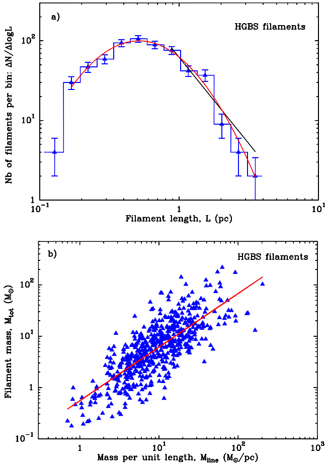
Fig. A.1. Panel a: differential distribution of lengths for the sample of 599 robust HGBS filaments identified by Arzoumanian et al. (2019). The red curve shows a lognormal fit to the overall distribution, the black solid line segment a power-law fit for filaments longer than 0.9 pc. Panel b: total mass M_{\text{tot}} against average mass per unit length M_{\text{line}} for the same sample of filaments as in the top panel. A strong linear correlation is observed between \log M_{\text{tot}} and \log M_{\text{line}} (with a Pearson correlation coefficient of \sim 77\% ). The red line shows the best-fit linear relation, M_{\text{tot}} = M_{\text{line}} \times L_{\text{eff}} , consistent with a typical effective length L_{\text{eff}} \sim 0.55 pc in the filament sample of Arzoumanian et al. (2019).
