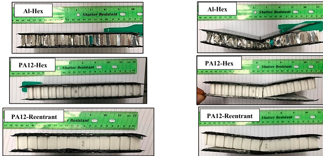
Fig. 2. Fabricated sandwiches before (left) and after (right) the bending test.
