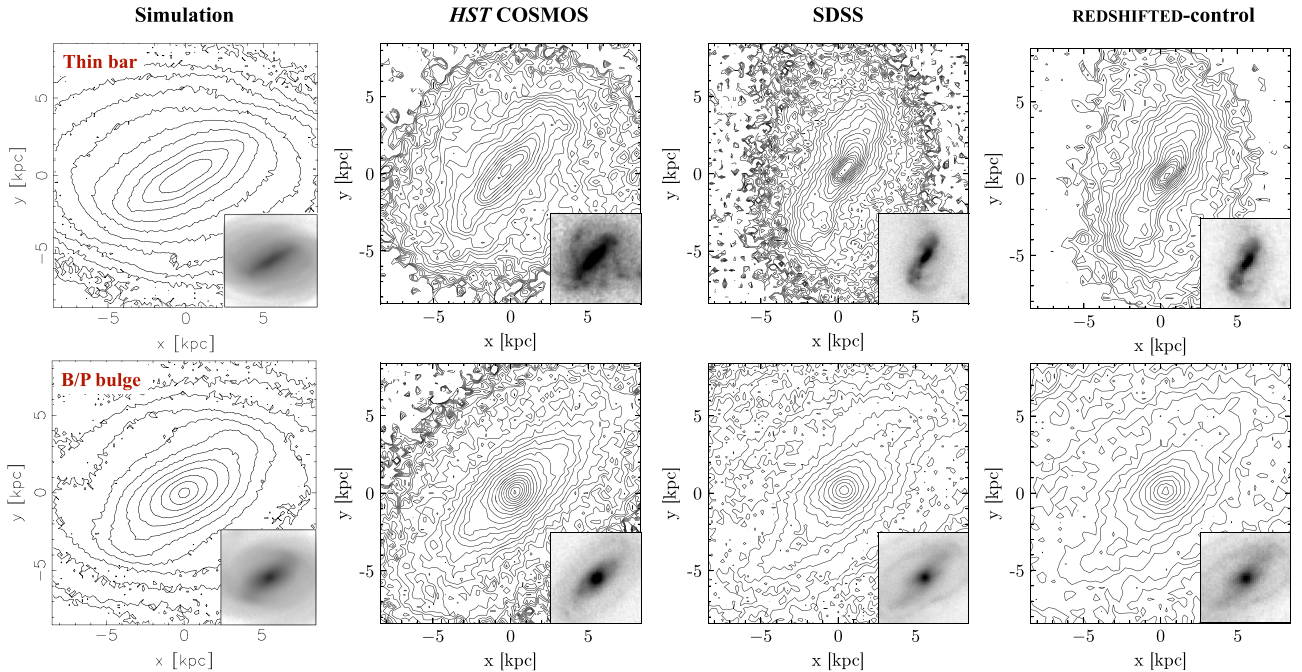
Figure 5. Top row: Example of a thin bar (No detected B/P bulge) from N -body simulations (Debattista et al. 2017), HST COSMOS, SDSS and REDSHIFTED-control SDSS data. Bottom row: Example of a B/P bulge from N -body simulations (Debattista et al. 2017) and B/P bulges as identified in COSMOS and SDSS data, following the typical isophotes – boxy isophotes in the centre and offset spurs on either side of the rectangle. The subplots at the bottom right show the original images of the galaxies from which the contour plots were derived, with an arcsinh stretch applied to the flux.
