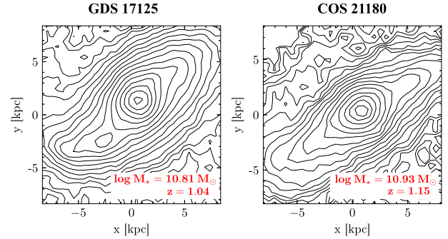
Figure B1. Two galaxies possibly hosting B/P bulges at z \gtrsim 1 , identified in the HST CANDELS survey, in the H band.
