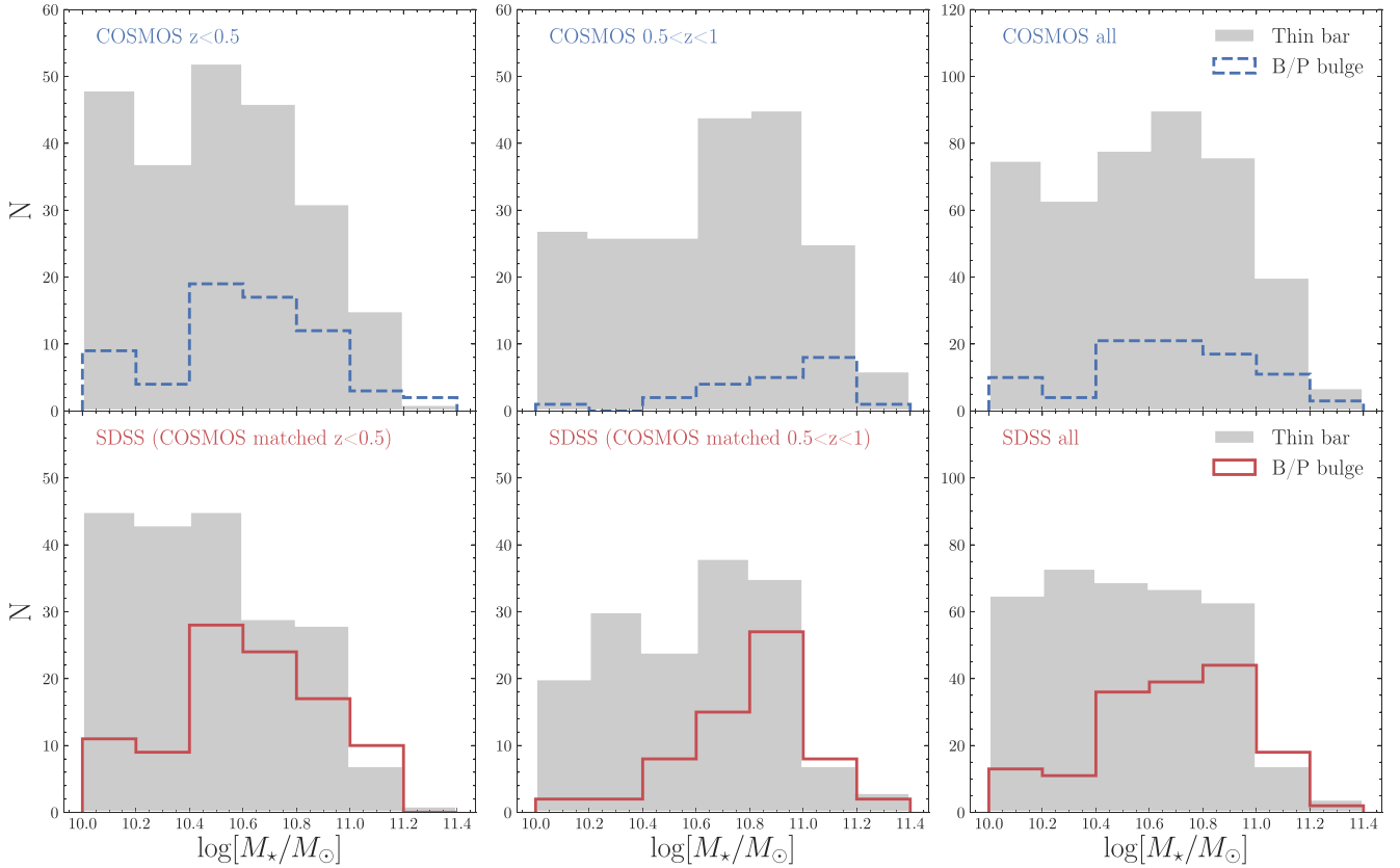
Figure 11. Distribution of stellar masses for galaxies classified as having B/P bulges and thin bars in the COSMOS sample, split into two redshift bins, z < 0.5 (top left panel) and 0.5 < z < 1 (top middle panel), as well as for the entire COSMOS sample (top right panel). For comparison, the stellar mass distribution of the B/P bulges and thin bars in the matched original SDSS data set, split into the same redshift bins of the corresponding COSMOS galaxies (bottom panels). The stellar mass distributions of B/P bulges and thin bars are remarkably similar for the COSMOS and SDSS galaxies, within the same redshift bin. The right-hand panels show the distribution of B/P bulges and thin bars in the entire COSMOS and SDSS data sets, respectively.
