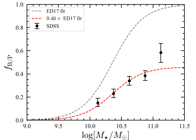
Figure 12. Detected frequency of B/P bulges in SDSS data set (black points), along with the original logistic fit for the ED17 local sample (gray dashed curve) and the same multiplied by our estimated detection efficiency for the SDSS data set of 46 per cent (red dashed curve).
