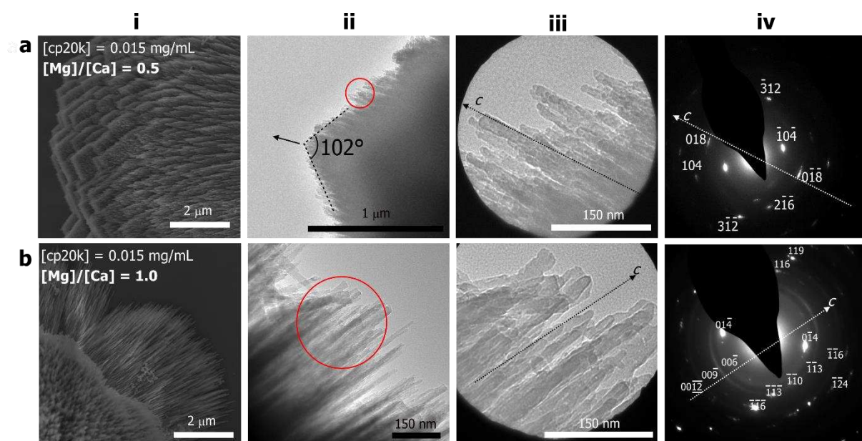
Figure 6: Characterization of calcite nanoshoots produced under CDM growth conditions with [cp20k] = 0.015 mg/mL and [\text{Mg}^{2+}]/[\text{Ca}^{2+}] = 0.5 ( a ) or 1.0 ( b ). i ) Representative SEM micrograph. ii ) Low magnification TEM micrograph of the edge of a fractured crystal. iii ) TEM micrograph of nanoshoots taken from area circled in red in ii . iv ) SAED of area shown in iii . Both iii and iv are annotated with the crystallographic c axis as determined from SAED.
