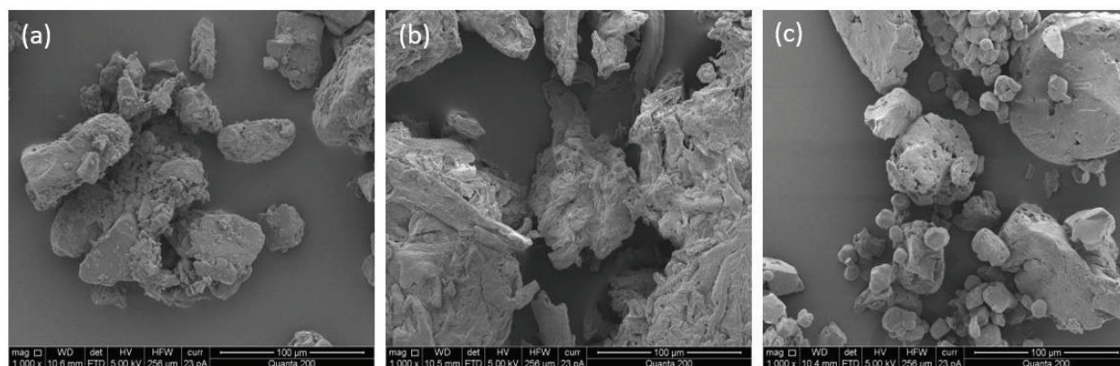
Figures 1. Images of coarse carbohydrate carriers i.e. (a) lactose monohydrate, LMH, (b) microcrystalline cellulose, MCC and, (c) Starch; for protransfersome powder formulations. These images are typical of four different experiment
