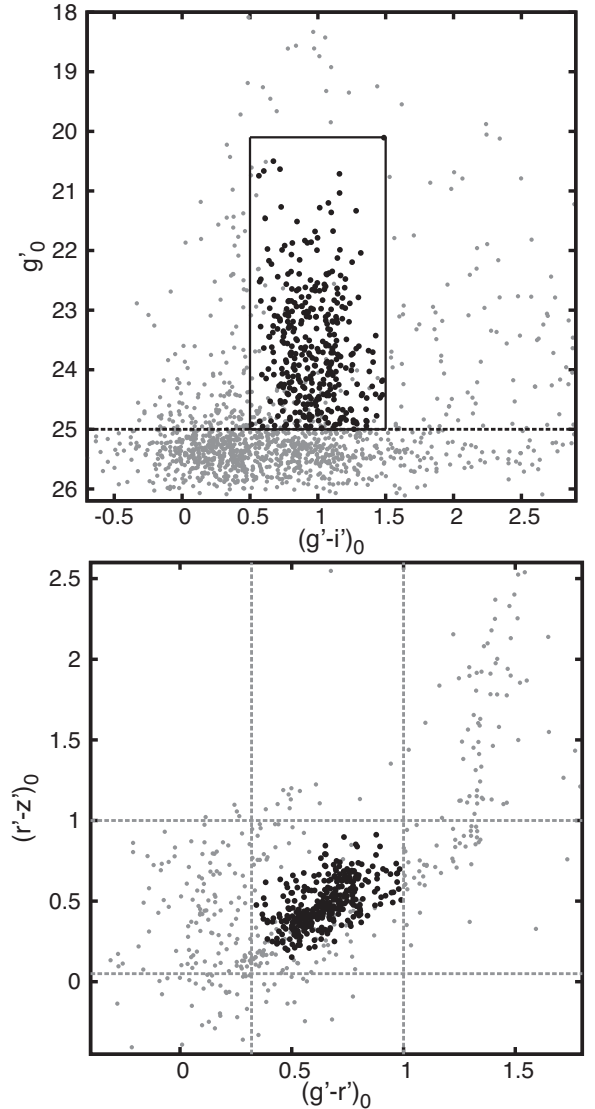
Figure 8. Upper panel: colour–magnitude diagram with all the unresolved sources detected in our GMOS mosaic (grey dots), as well as our final sample of GC candidates (black dots inside the box). The horizontal dashed line indicates the magnitude corresponding to \epsilon_{(g' - i')} \sim 0.1 mag. Bottom panel: colour–colour diagram with the unresolved sources brighter than g'_0 = 25 mag. The dashed grey lines show the colour ranges considered for the selection of GC candidates.
