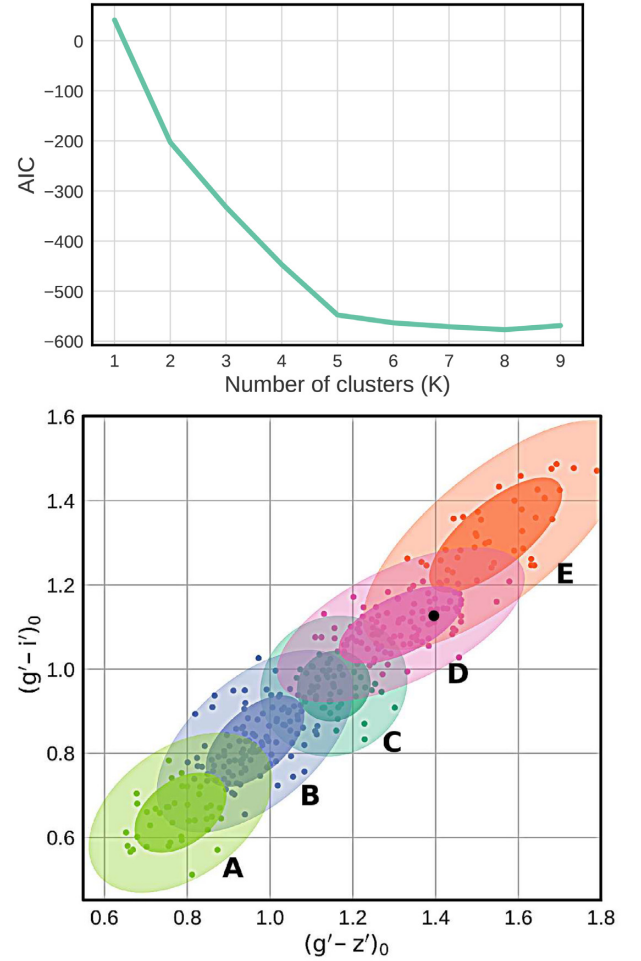
Figure 10. Upper panel: AIC as a function of the number of the fitted Gaussian components ( K ). Bottom panel: Colour–colour diagram background-corrected with the five-considered Gaussian components. The small and large ellipses represent 68 percent and 95 percent confidence intervals of the different Gaussian components, respectively. The black filled circle indicates the position of the UCD.
