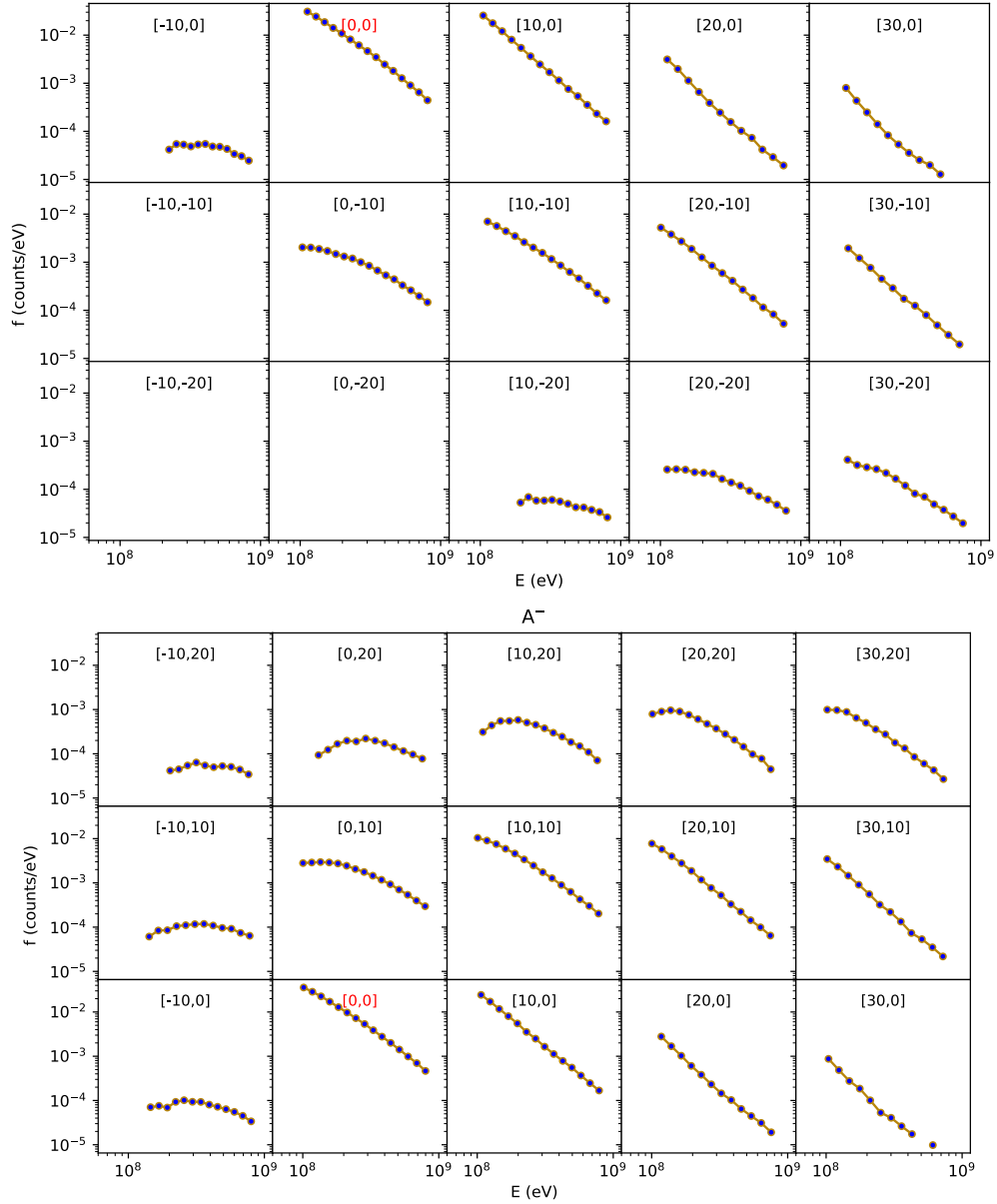
Fig. 4. Fluence energy spectra for A^+ (top) and A^- (bottom) configurations of the IMF, at a variety of 1 AU locations with respect to the best connected location ([0, 0]) , for a power law population. The solid lines in the [0, 0] panels give the slope of the injection spectrum. Parameters of the simulations are as in Fig. 3.
