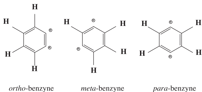
Figure 2. Structure of ortho-, meta-, and para-benzynes.
