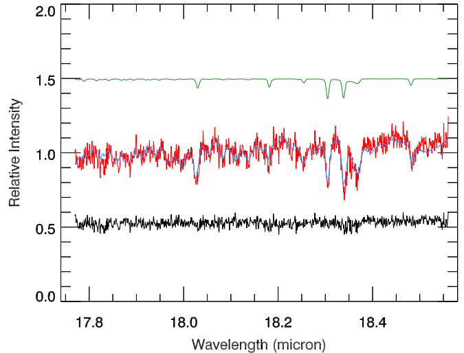
Figure 1. SOFIA/EXES spectra of V4334 Sgr in the 18 \mu\text{m} region near the 18.28 \mu\text{m} in-plane aromatic ring deformation of benzyne ( \text{C}_6\text{H}_4 ) observed in terrestrial laboratories. The V4334 Sgr spectrum is the red curve, the mean-normalized Callisto (the telluric divisor) spectrum is the blue curve, and the black curve is the division of the two observed spectra multiplied by a factor of 100. The green curve is the ATRAN (Lord 1992) transmission model (arbitrarily offset by a factor of 0.5 for clarity). The spectral grasp of our observations does not include the 17.4 \mu\text{m} region in the blue, nor extend to the 18.9 \mu\text{m} region in the red where \text{C}_{60} fullerene features are sometimes seen in the dust continuum of objects exhibiting PAH and other UIR bands (Shannon et al. 2015, and references therein).
