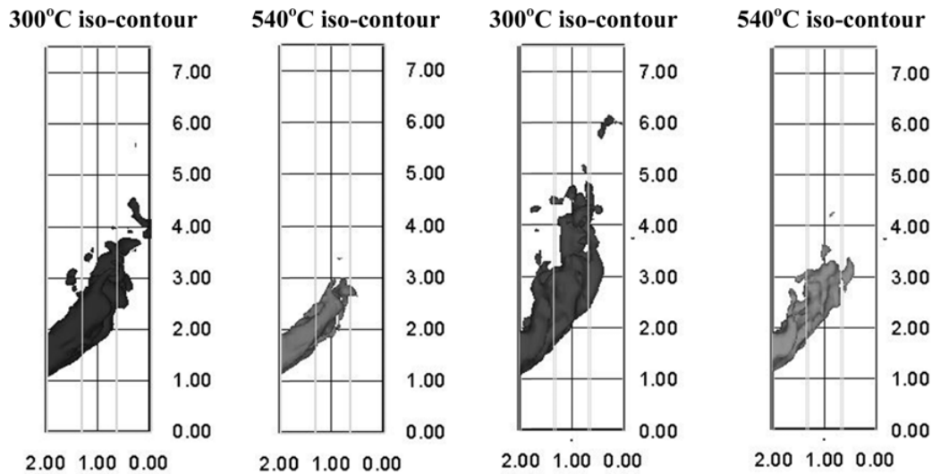
Figure 10. Predictions of 300°C and 540°C iso-contours for the NoFD (left) and FD (right) test case.
