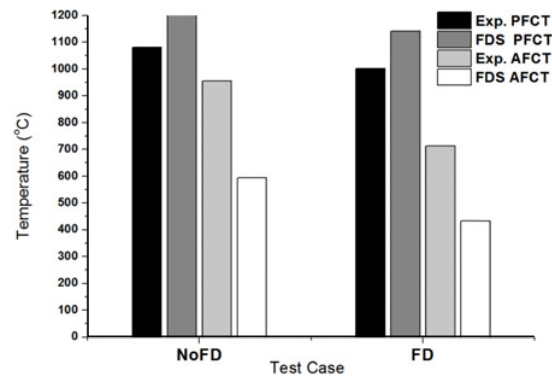
Figure 6. Peak Fire Compartment Temperatures (PFCT) and Average Fire Compartment Temperatures (AFCT) for the NoFD (left) and FD (right) test cases.
