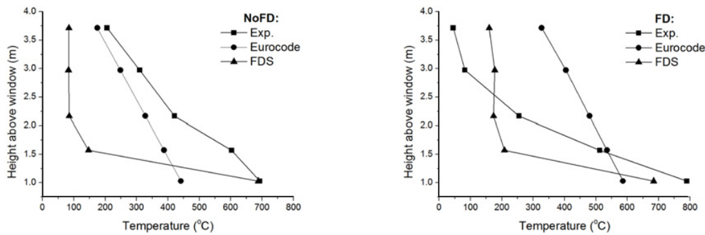
Figure 9. Centreline EVF temperatures in the NoFD (left) and FD (right) test case.
