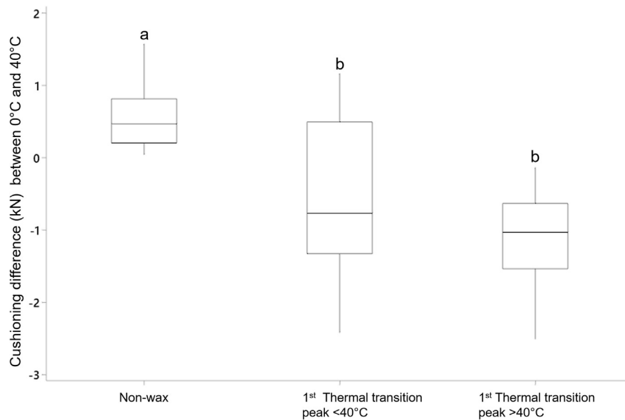
Fig. 3 – Overall difference in cushioning (kN) between 0 °C and 40 °C. Surfaces were categorised as Non-wax; 1st thermal transition peak <40 °C and 1st thermal transition peak >40 °C. Greater range in cushioning was seen in 1st thermal transition peak <40 °C and 1st thermal transition peak >40 °C than in Non-wax ( H_2 = 9.42 P = 0.009 ). Interquartile range and median have been demonstrated.
