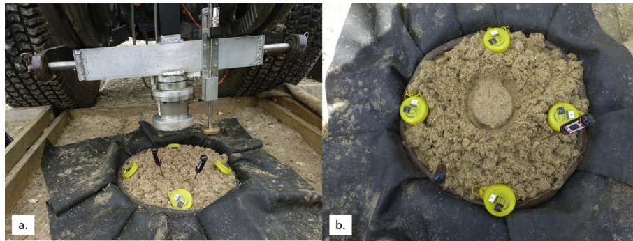
Fig. 1 – Racetrack surfaces were prepared in latex-lined moulds embedded in test boxes. (A) Temperature was continuously measured using Tinytag™ Transit 2 (Model: TG-4080) data-loggers. (B) The imprint of the hoof occurred after each surface testing device was dropped. The Orono Biomechanical Surface Tester is depicted in this specific image.
