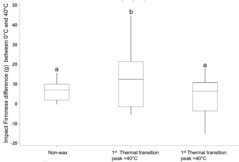
Fig. 4 – Overall difference in impact firmness (g) between 0 °C and 40 °C. Surfaces were categorised as Non-wax; 1st thermal transition peak <40 °C and 1st thermal transition peak >40 °C. Greater range in impact firmness was seen in 1st thermal transition peak <40 °C ( F_{2, 81} = 8.20 ; R^2 = 25.81\% P = 0.001 ). Interquartile range and median have been demonstrated.
