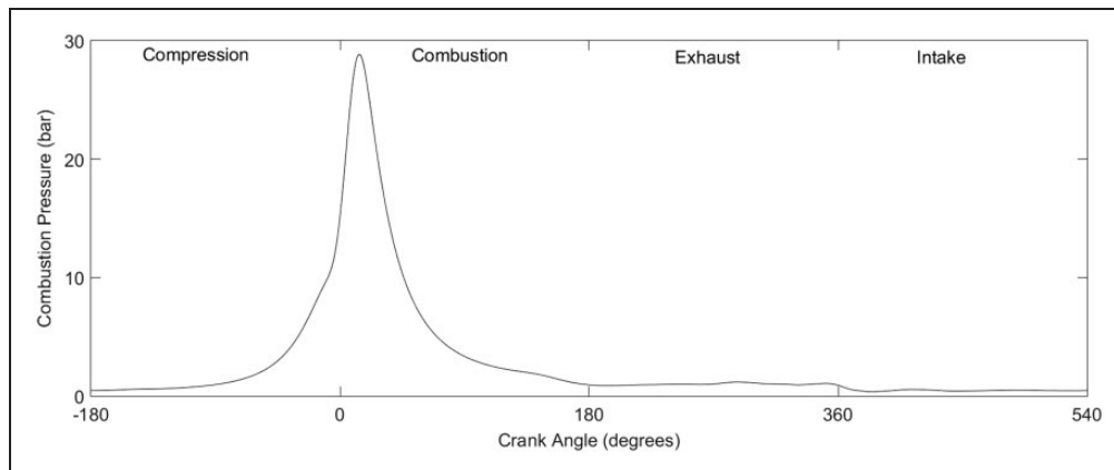
Figure 6. Combustion pressure.
