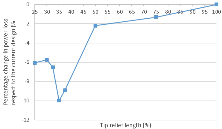
Figure 13: Percentage change in power loss with respect to the current design for the 25% - 100% (current design) tip relief length cases surface roughness of 1.6 \mu m)
