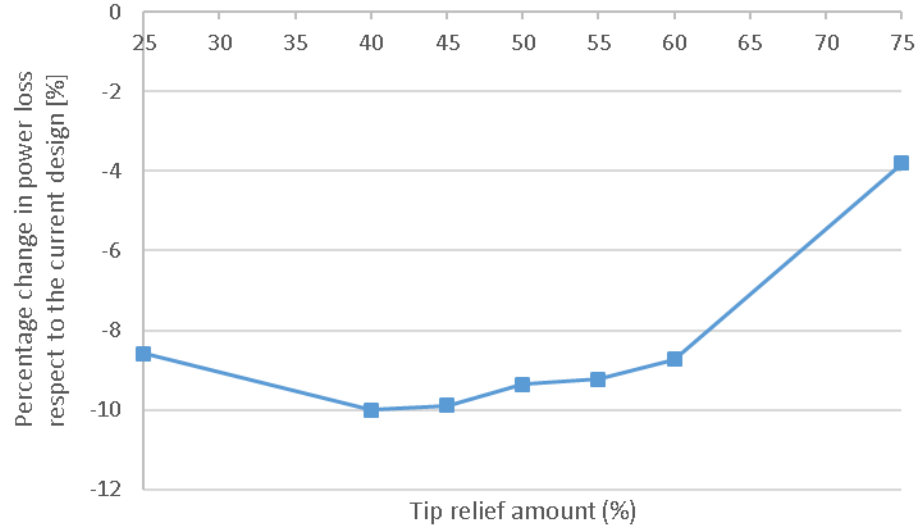
Figure 9: Percentage change in power loss with respect to the current design for 25% - 75% tip relief amount (with surface roughness of 1.6\mu\text{m} )
