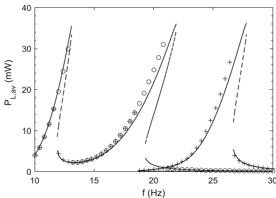
Fig. 11 Average power P_{L,av} of electrical load with R_L = 1k\Omega for the parameters of Fig. 6 and electrical damping, c_{el} = 0.0456 Ns/m. Stable (solid line) and unstable (dashed line) analytical solution from Eq. (12a-c); (circle) forward sweep from numerical integration of Eq. (4) and (plus) backward sweep
