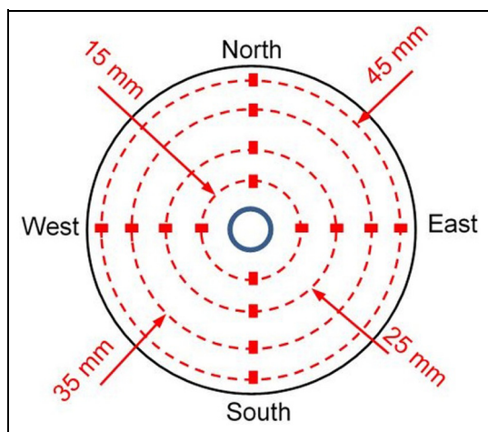
Figure 9. The sliding tracks and the locations of surface interferometric measurements (small rectangular areas at North, West, South and East).
