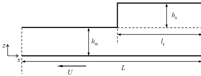
Fig. 8. Schematic of Rayleigh step bearing.
